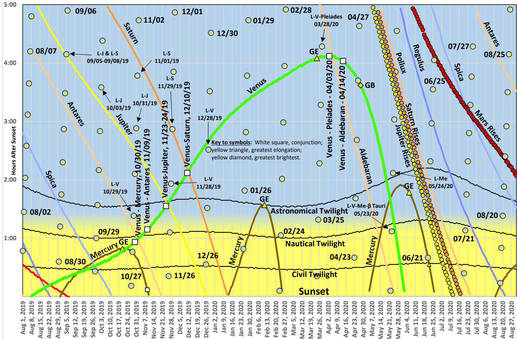
All moon dots, and the curves for planets and stars, indicate setting times in relation to sunset, except for the three planet curves labeled to indicate times of rising, also in relation to sunset.
