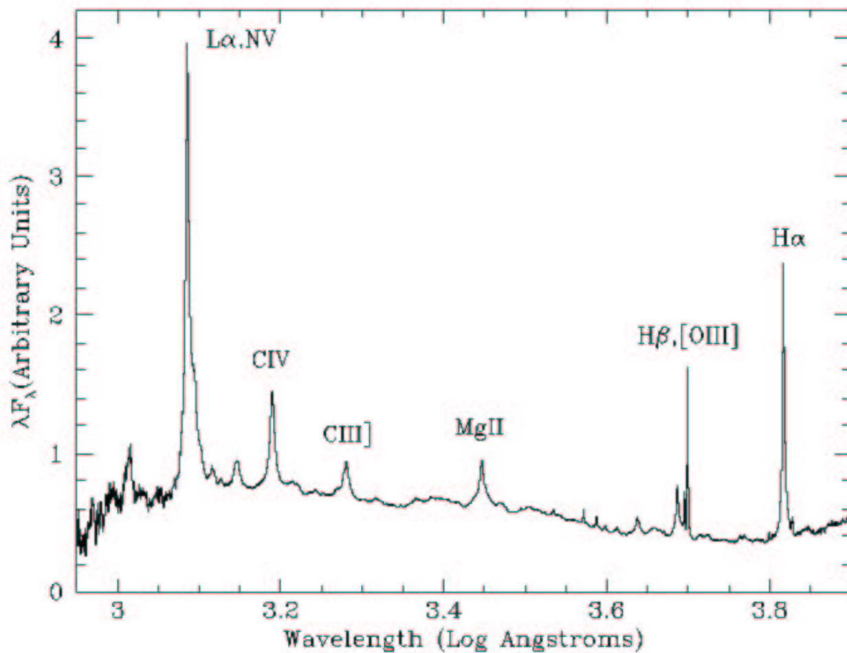
FIG. 1.— FBQS composite spectrum plotted as \lambda F_{\lambda} vs. the logarithm of the rest-frame wavelength. Prominent emission features are marked. The y-axis has been normalized such that the spectrum has values on order of unity.
