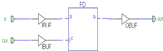
Figure 4-2 MACROS2 Schematic
