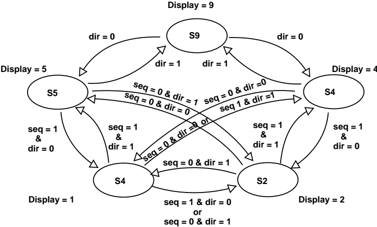
Figure 7-1 State Diagram
