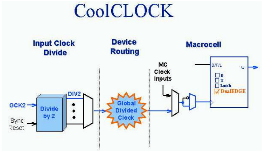
Figure 2.32 CoolCLOCK
