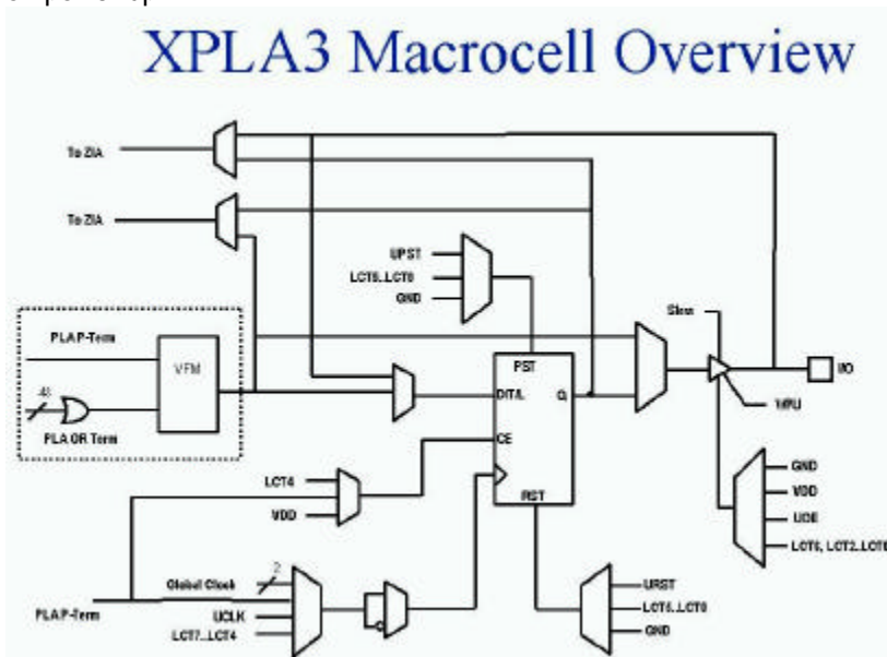
Figure 2.21 CoolRunner XPLA3 Macrocell Diagram
