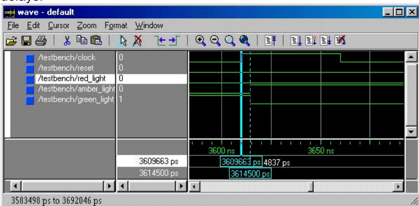
Figure 6.5.1 Simulation Waveform
