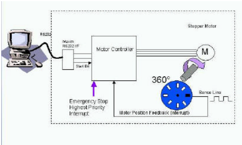
Figure 7.2.5 Design Partitioning
