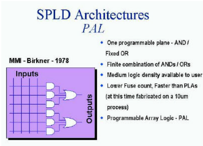
Figure 1.2 SPLD Architectures
