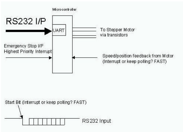
Figure 7.2.6 Microcontroller Implementation
