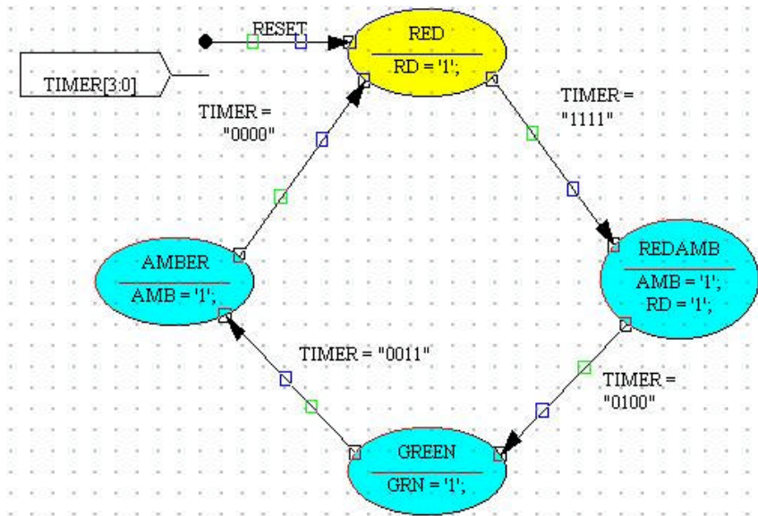
Figure 4.4.8 State Machine Drawing
