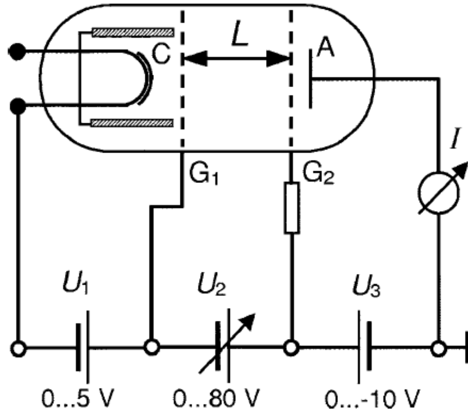
Fig. 1. Schematic diagram of the Franck-Hertz experiment.
