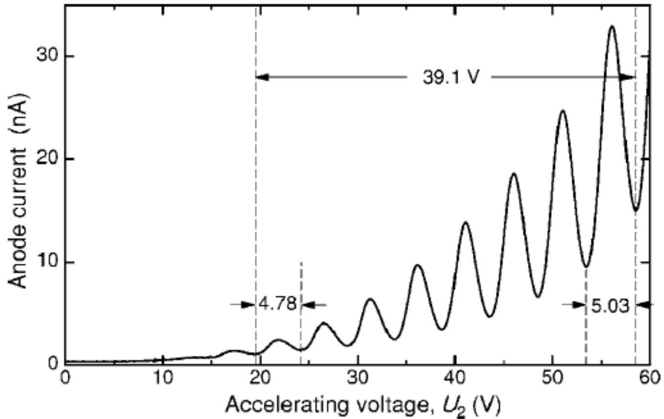
Fig. 3. Typical Franck-Hertz curve recorded with Hg tube at 170 °C.
