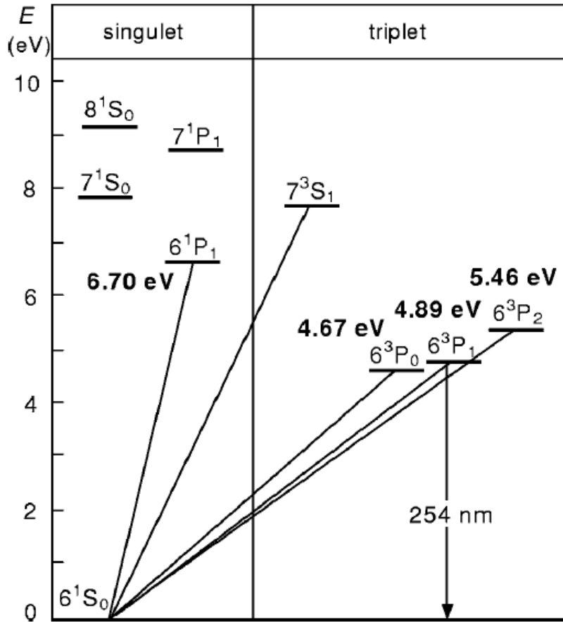
Fig. 2. Lowest energy levels in Hg (Ref. 10).
