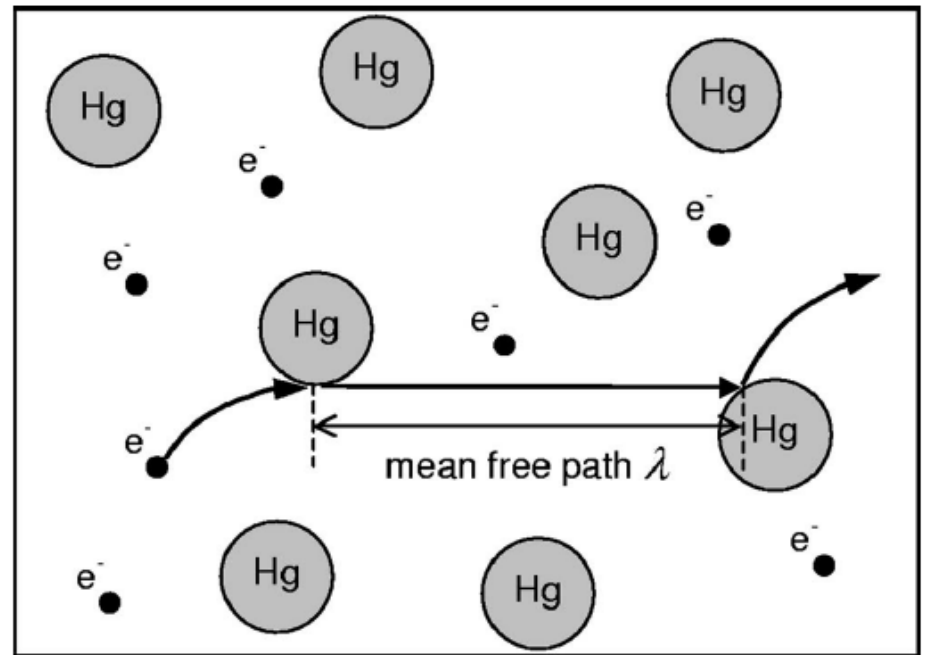
Fig. 5. Schematic of the energy transfer from electrons to atoms.
