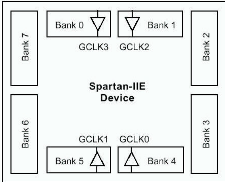
Figure 2.7 Spartan IIE Banking of I/O Standards
