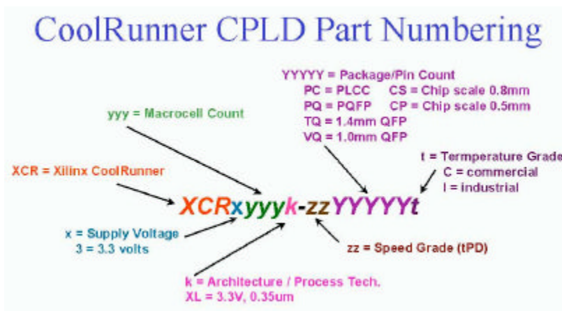
Figure 2.24 CoolRunner XPLA3 Part Number System
