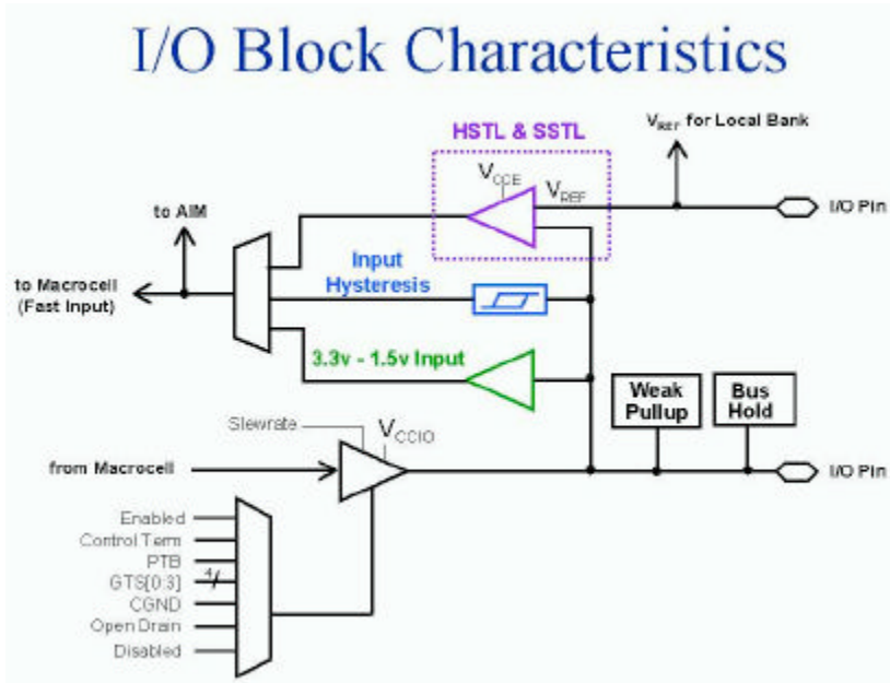
Figure 2.29 CoolRunner II I/O Block
