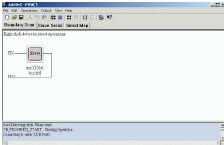
Figure 6.6.1 iMPACT Programmer Main Window
