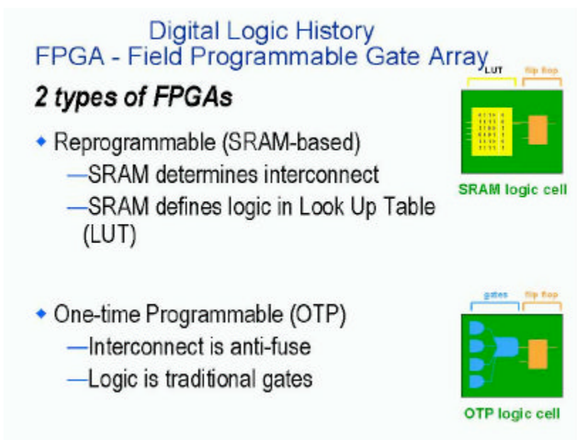
Figure 1.5 Digital Logic History
