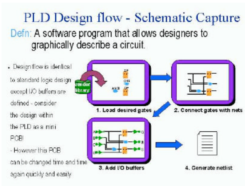
Figure 1.7 PLD Design Flow
