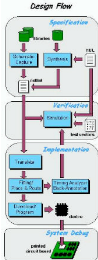
Figure 1.10 The PLD Design Flow
