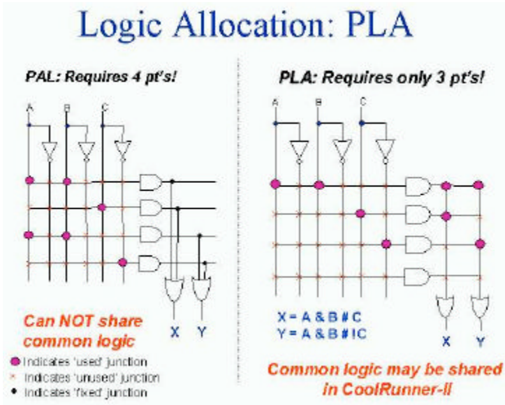
Figure 2.27 Logic Allocation – Typical PAL vs. PLA
