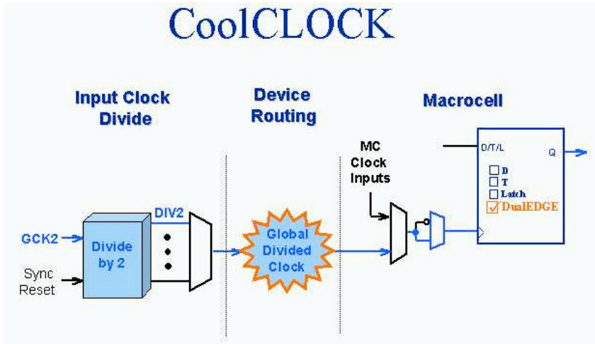
Figure 2.32 CoolCLOCK
