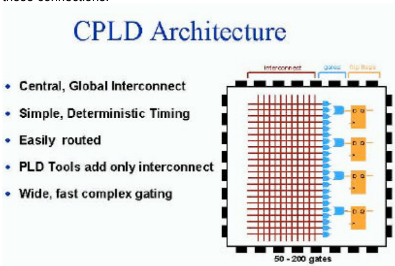
Figure 1.3 CPLD Architecture
