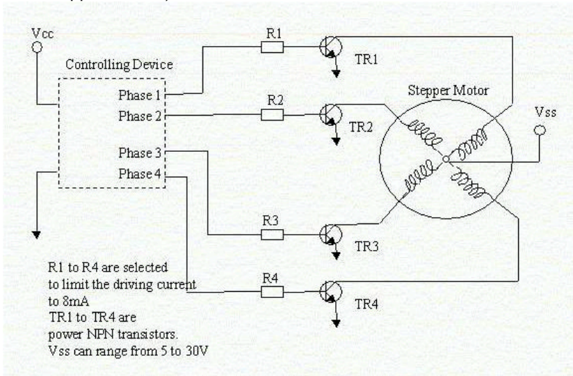
Figure 7.2.1 Stepper Motor Controller
