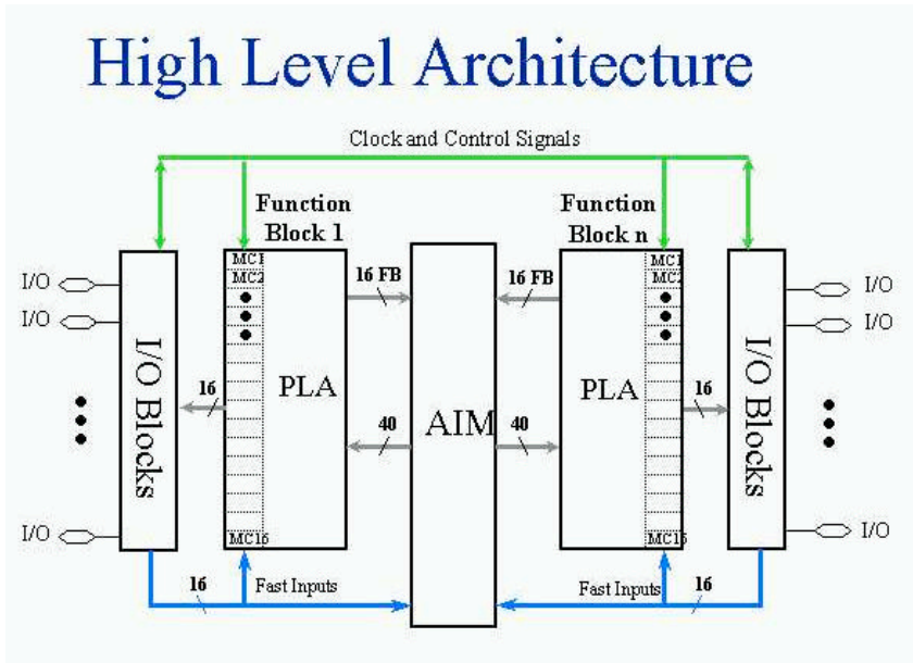
Figure 2.26 CoolRunner II High Level Architecture
