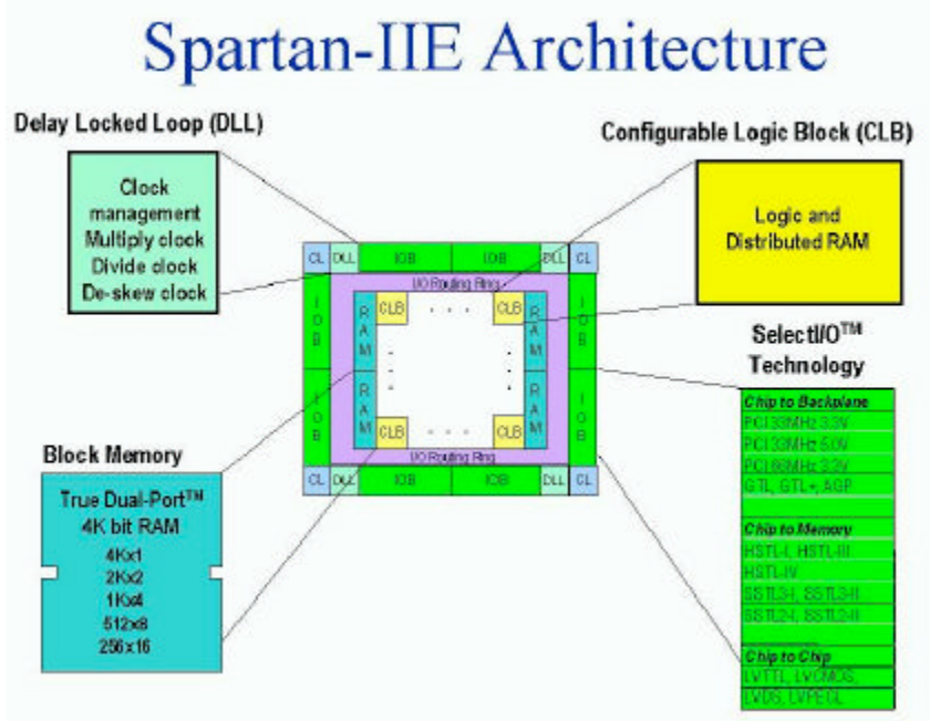
Figure 2.4 Spartan IIE Architecture
