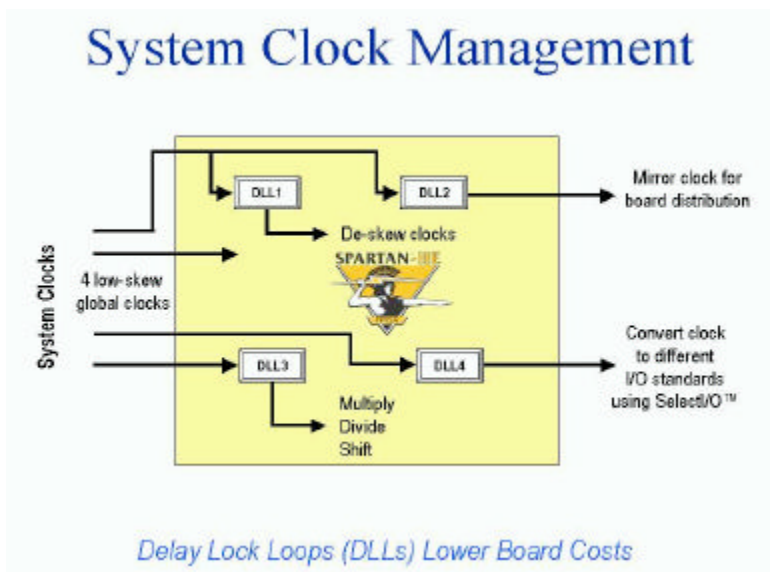
Figure 2.11 Spartan IIE Clock Management
