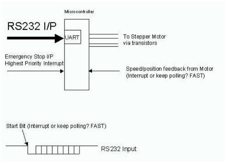
Figure 7.2.6 Microcontroller Implementation
