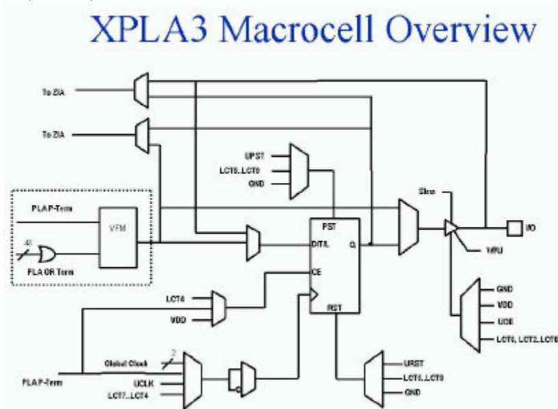
Figure 2.21 CoolRunner XPLA3 Macrocell Diagram
