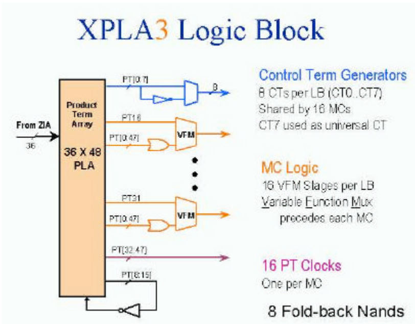
Figure 2.20 CoolRunner XPLA3 Logic Block
