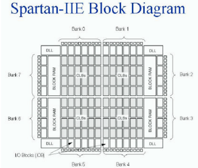
Figure 2.5 Spartan IIE Block Diagram
