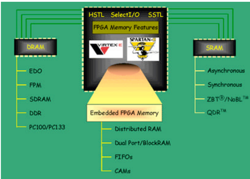
Figure 2.5.7 Memory Solutions on the Xilinx Website
