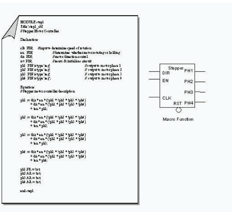
Figure 7.2.4 CPLD ABEL program to control a stepper motor
