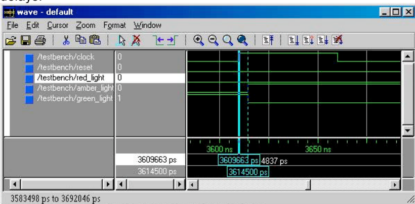
Figure 6.5.1 Simulation Waveform
