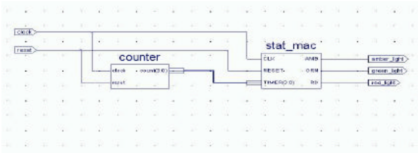
Figure 4.6.7 Adding I/O markers
