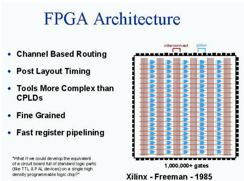
Figure 1.4 FPGA Architecture
