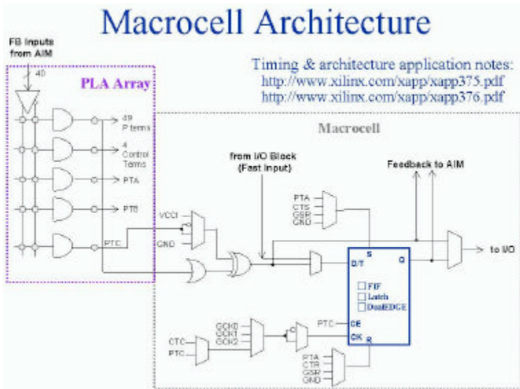
Figure 2.28 CoolRunner II Macrocell
