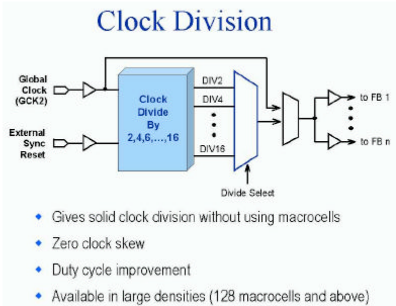
Figure 2.31 CoolRunner II Clock Division
