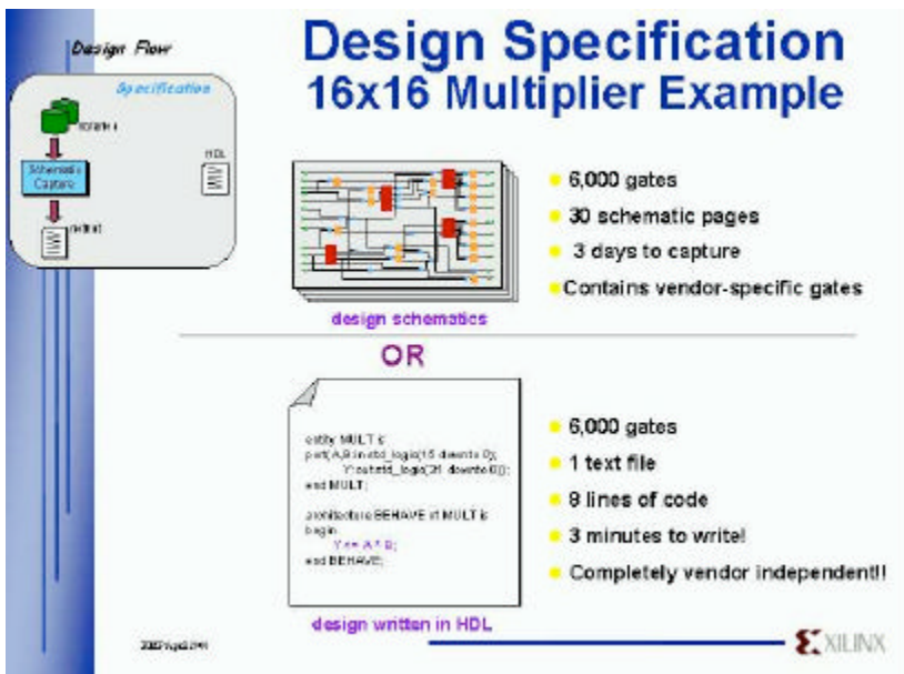
Figure 1.9 Design Specification – Multiplier
