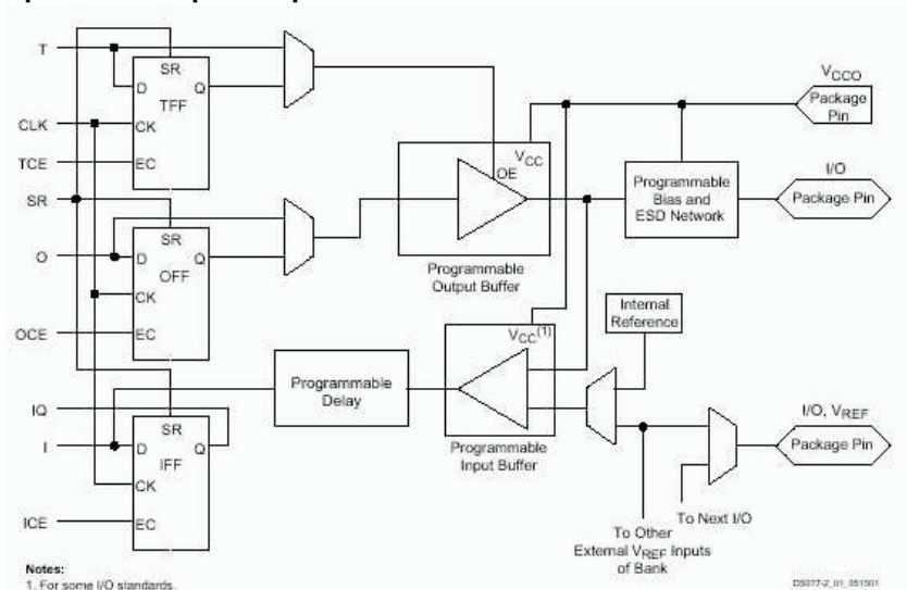
Figure 2.6 Spartan IIE Input/Output Block
