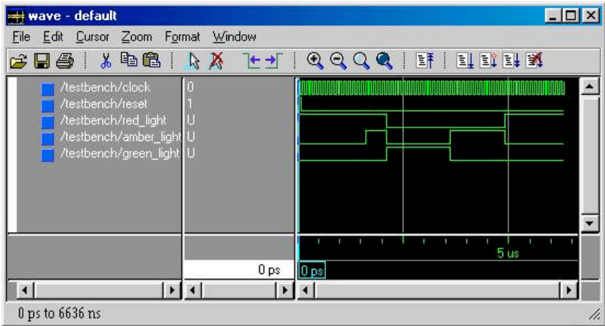
Figure 4.5.8 Waveform Window
