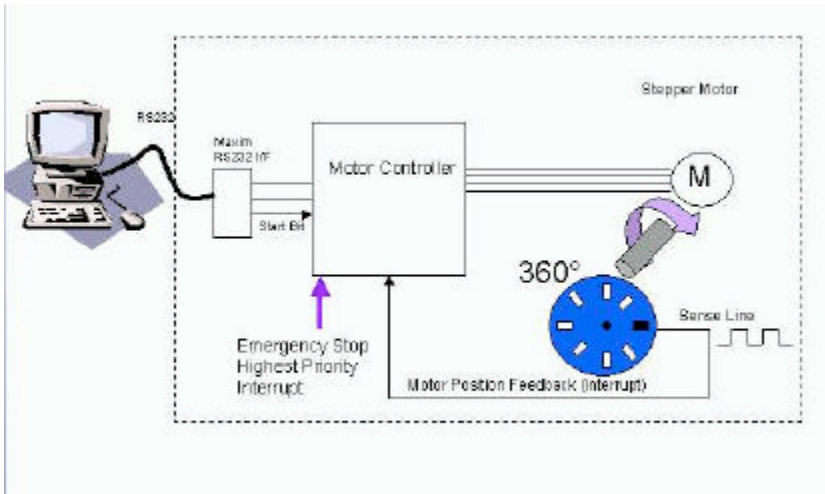
Figure 7.2.5 Design Partitioning
