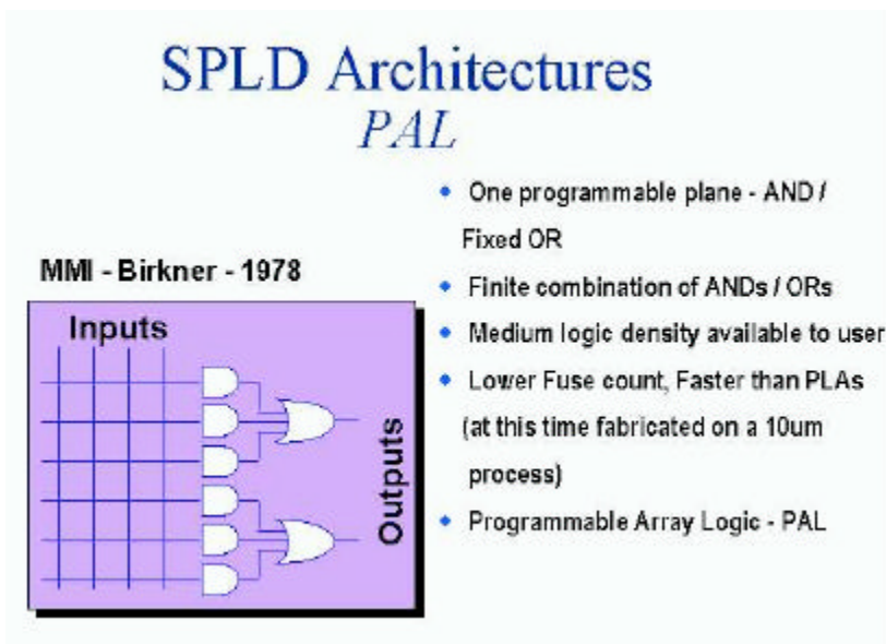
Figure 1.2 SPLD Architectures
