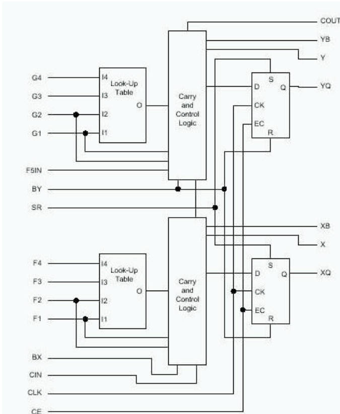
Figure 2.8 Spartan IIE Logic Cell
