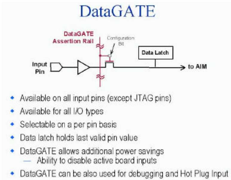
Figure 2.30 DataGATE Function in CoolRunner II
