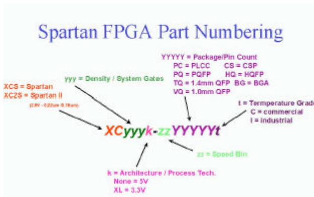
Figure 2.14 Spartan FPGA Part Numbering Guide
