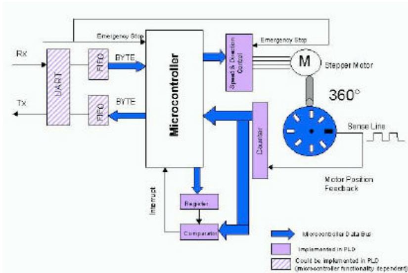
Figure 7.2.7 Partitioned Design: Microcontroller and CPLD
