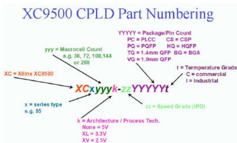
Figure 2.16 XC9500 CPLD Part Numbering System
