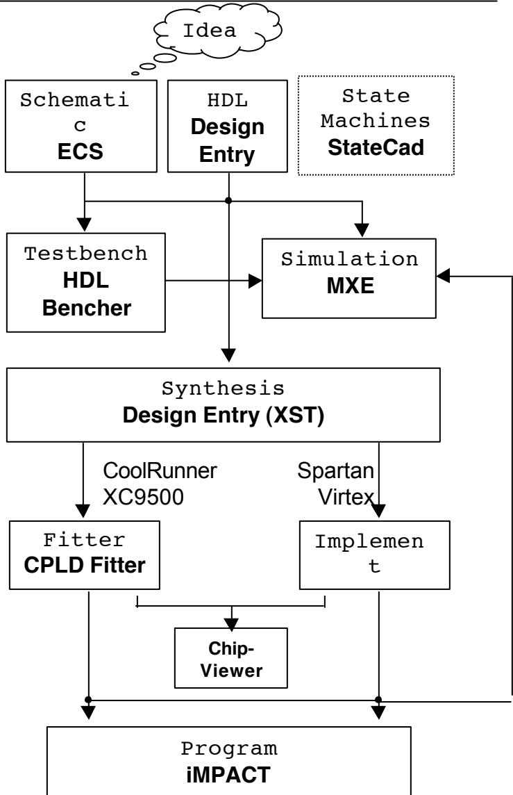
Figure 3.1 WebPACK Design Flow
