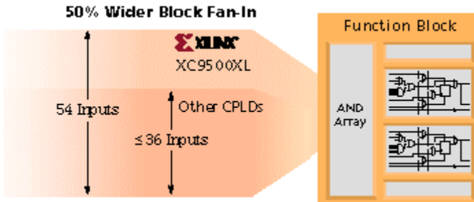
Figure 2.15 XC9500XL Block Fan-In
