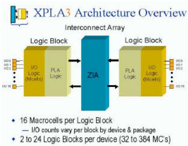
Figure 2.19 CoolRunner XPLA3 Architecture Overview
