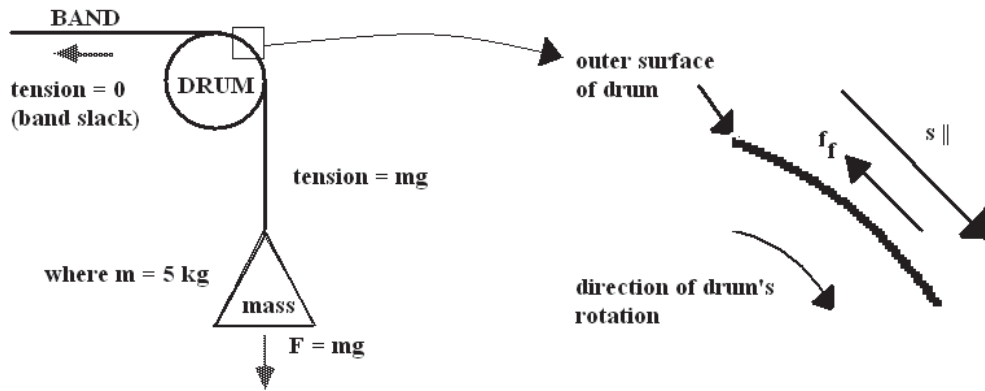
Figure 6.2: Diagram of f_f and s_{||} .
