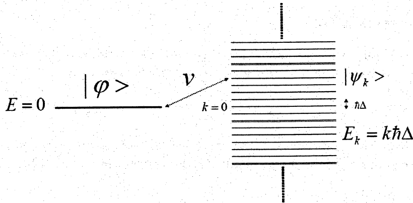
Figure 1: Spectrum of H_0 . The states |\varphi\rangle represents a quasi bound state with energy E = 0 whereas |\psi_k\rangle denotes an infinite set of equally spaced states with energy E_k = k\hbar\Delta where k is a positive or a negative integer.
