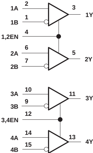
SN65LVDS3486D logic diagram (positive logic)
