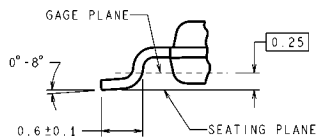
DETAIL A TYPICAL
