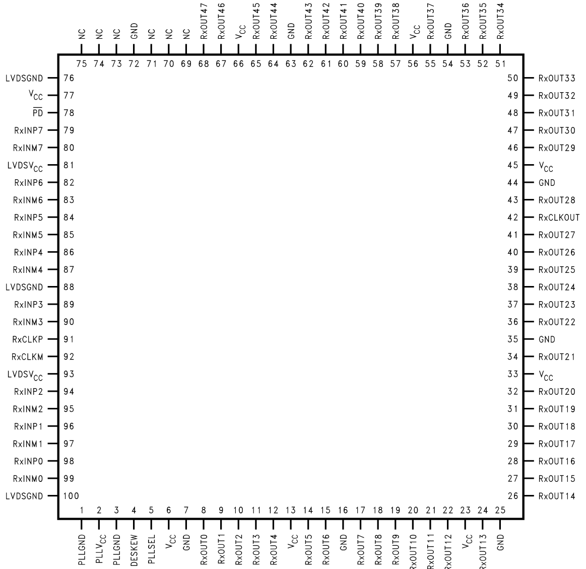
Receiver - DS90CR484 - TQFP (TOP VIEW)
