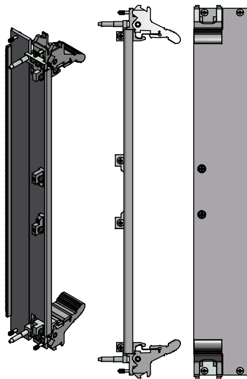
6U 8HP Ejector and Attached Center PCB Mounts
