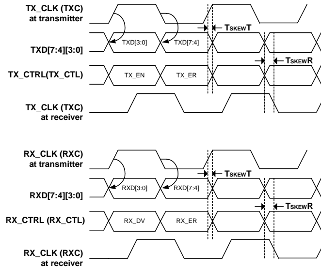
Figure 24: RGMII Multiplexing and Timing
