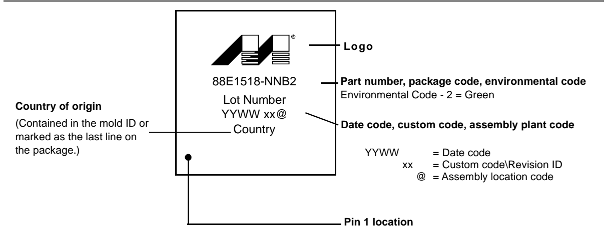
Figure 39: 88E1518 48-pin QFN Commercial Green Compliant Package Marking and Pin 1 Location
