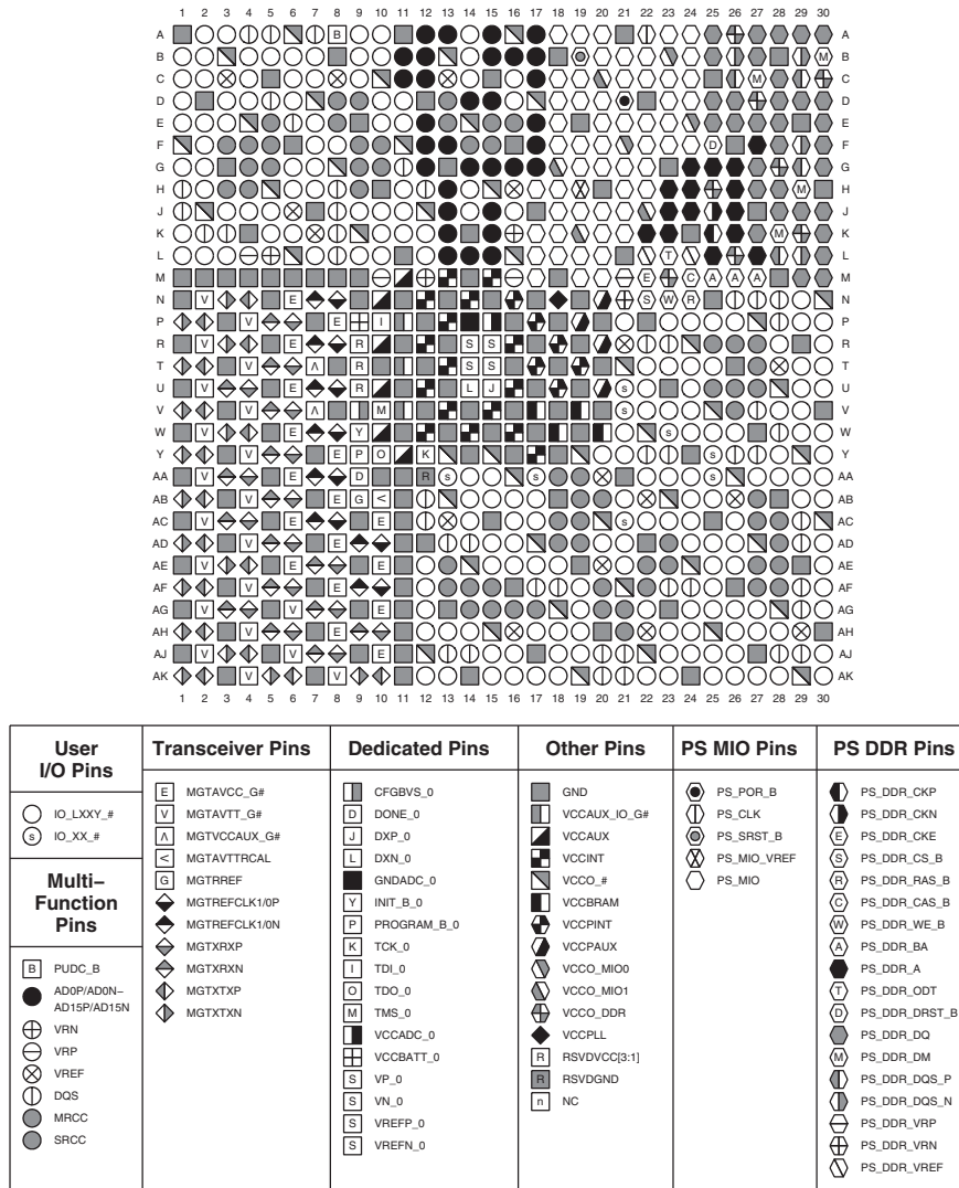
Figure 3-45: FF900/FFG900/FFV900/RF900 Packages—XC7Z035, XC7Z045, and XQ7Z045 Pinout Diagram
