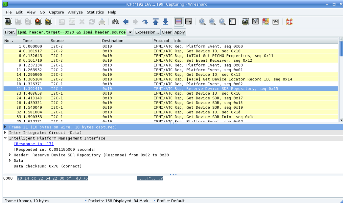
Figure 16 Filtered Trace
