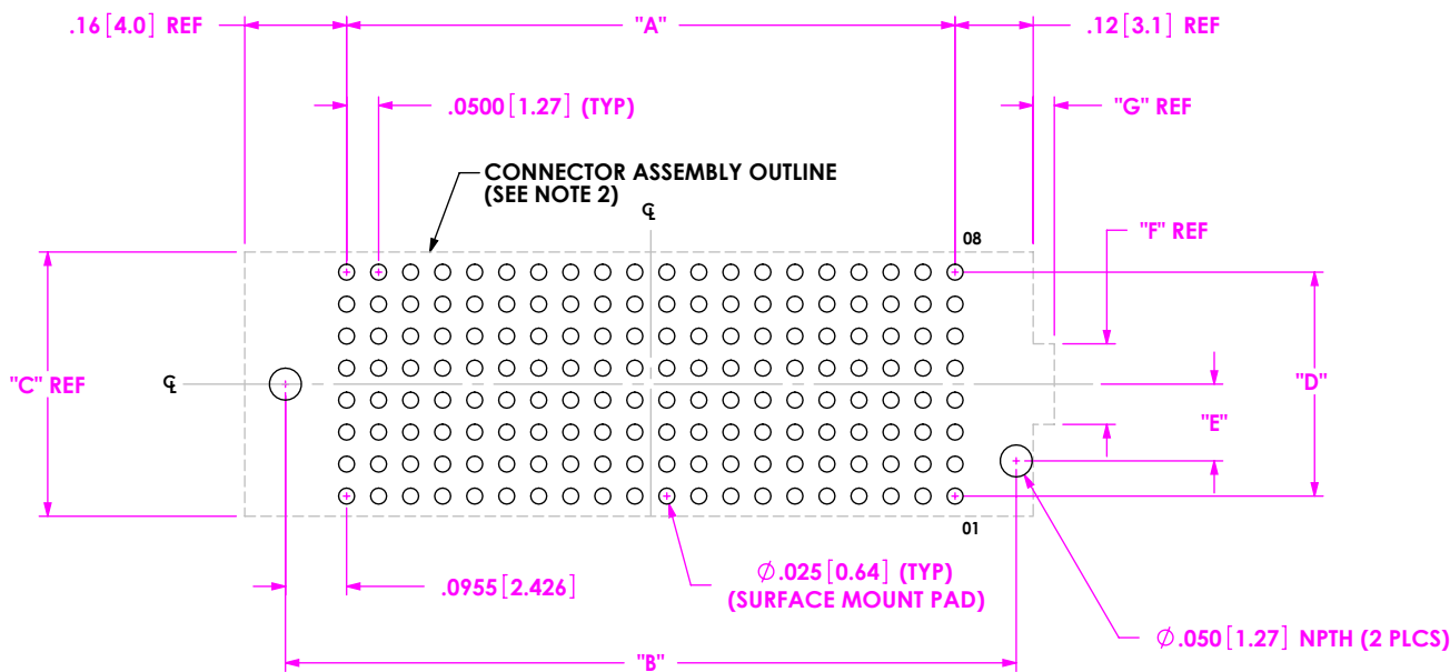
FIG. 1 FOOTPRINT FOR SEAF-20-XX.X-XX-08-X-A SHOWN
