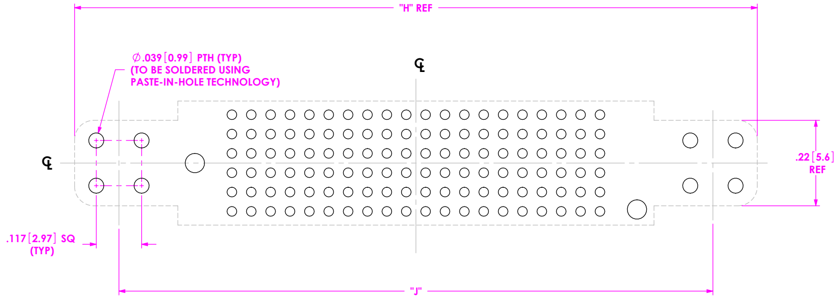
FIG. 5 -LP & -PP OPTION P FOOTPRINT FOR SEAF-20-XX.X-XX-06-X-A-LP SHOWN (SAME AS FIG. 1, EXCEPT AS SHOWN)
