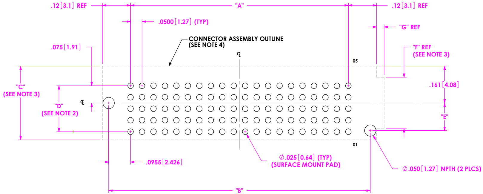
FIG. 3 FOOTPRINT FOR SEAF-20-XX.X-XX-05-X-A SHOWN
