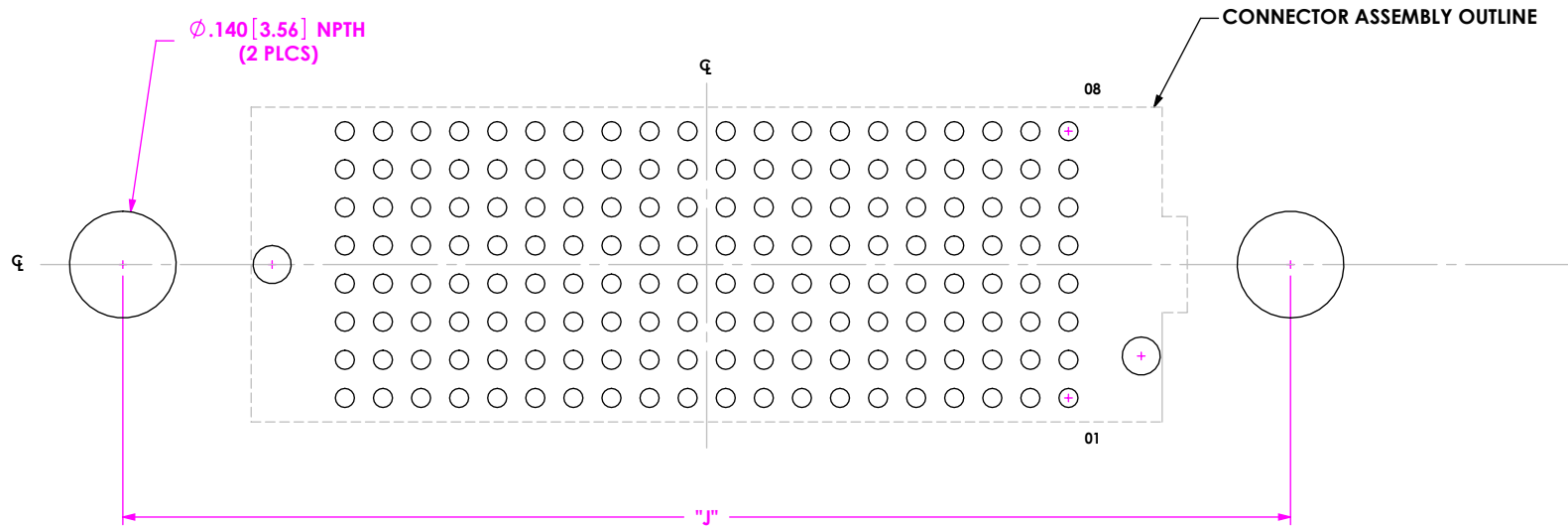
FIG. 7 -EP OPTION FOOTPRINT FOR SEAF-20-XX.X-XX-08-X-A-EP SHOWN (SAME AS SEAF-20-XX.X-XX-08-X-A, EXCEPT AS SHOWN) (NOT AVAILABLE WITH -LP OR -PP OPTIONS) (ONLY AVAILABLE IN 20, 30, 40 & 50 POSITIONS) (STENCIL LAYOUT SAME AS FIG. 2) (NOT RELEASED FOR PRODUCTION)
