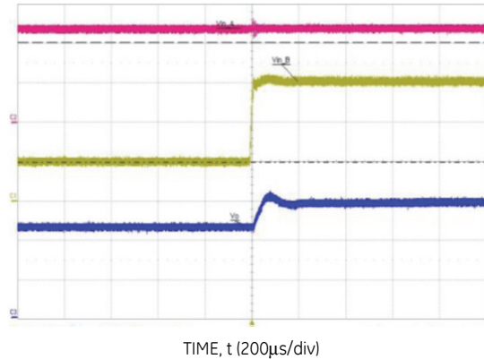
Fig 2: Input Transient on one feed CH1: Feed B step to 60V (20V/Div) CH2: Feed A at 48V (20V/Div) CH3: VRTN_OUT (20V/Div)
