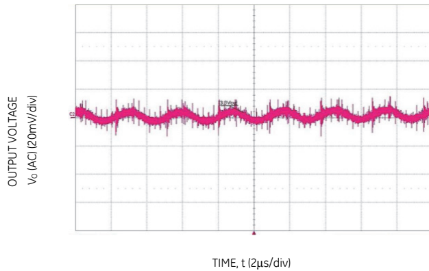
Fig 12: 3.3V Ripple
