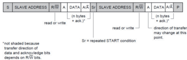
Fig 20: Typical I 2 C Read protocol
