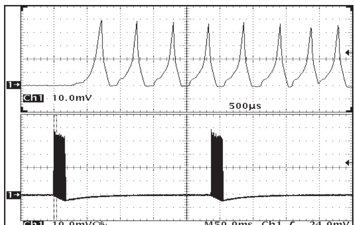
Figure 17: Load current (10 A/div) as a function of time when the converter attempts to turn on into a 1m\Omega short circuit. Top trace (500 μs/div) is an expansion of the on-time portion of the bottom trace.
