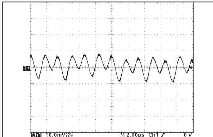
Figure 14: Input reflected ripple current, i_s , through a 5\mu H source inductor, using a 47\mu F electrolytic input capacitor (10 mA/div). See Figure 12.
