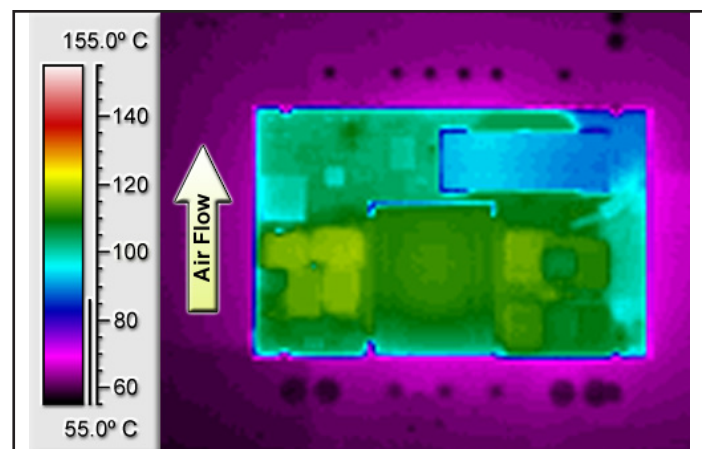
Figure 6: Thermal plot of converter at 23.3 A load current (279.6 W) with 55°C air flowing at the rate of 200 LFM. Air is flowing across the converter from pin 3 to pin 1 (nominal input voltage).
