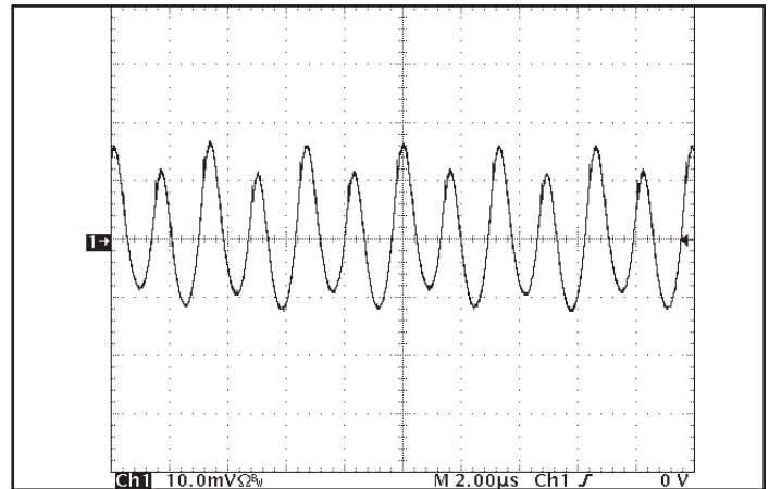
Figure 13: Input Terminal Ripple Current, i_c , at full rated output current and nominal input voltage with 5\mu H source impedance and 47\mu F electrolytic capacitor (500 mA/div). See Figure 12.
