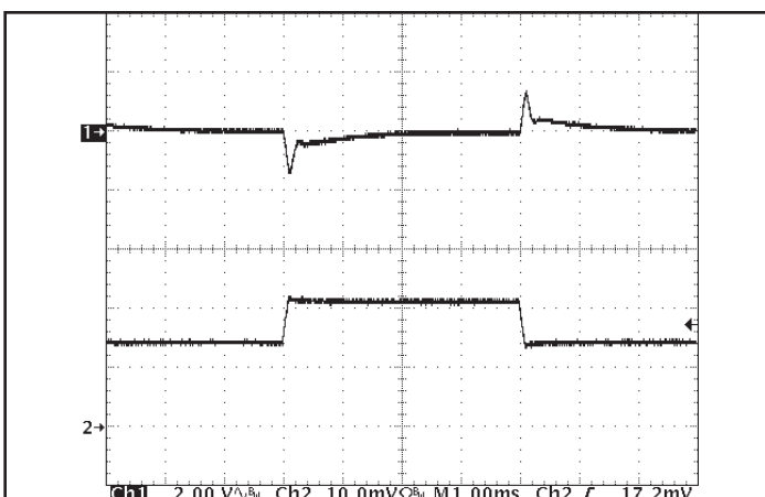
Figure 11: Output voltage response to step-change in load current (50%-75%-50% of Iout(max); dI/dt = 0.1A/μs). Load cap: 100 μF, 100 mΩ ESR tantalum cap and 1 μF ceramic cap. Ch 1: Vout (2 V/div), Ch 2: Iout (10A/div).
