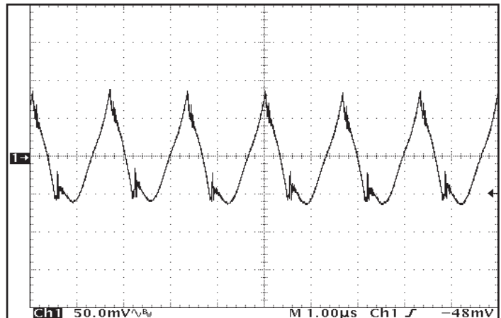
Figure 15: Output voltage ripple at nominal input voltage and rated load current (50 mV/div). Load capacitance: 1\mu F ceramic capacitor and 15\mu F tantalum capacitor. Bandwidth: 20 MHz. See Figure 12.
