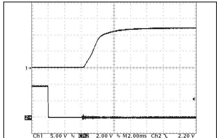
Figure 10: Turn-on transient at zero load (2 ms/div). Load cap: 3 mF output capacitance. Ch 1: Vout (5 V/div), Ch 2: ON/OFF input (2 V/div).
