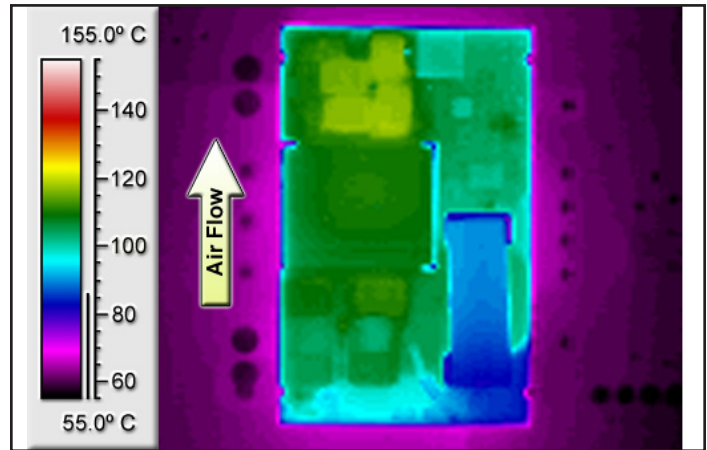
Figure 8: Thermal plot of converter at 21.9 A load current (262.8 W) with 55°C air flowing at the rate of 200 LFM. Air is flowing across the converter from output to input (nominal input voltage).
