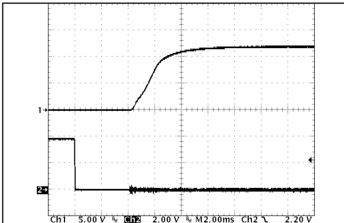
Figure 9: Turn-on transient at half load (resistive load) (2 ms/div). Load cap: 3 mF output capacitance. Input voltage pre-applied. Ch 1: Vout (5 V/div), Ch 2: ON/OFF input (2 V/div).
