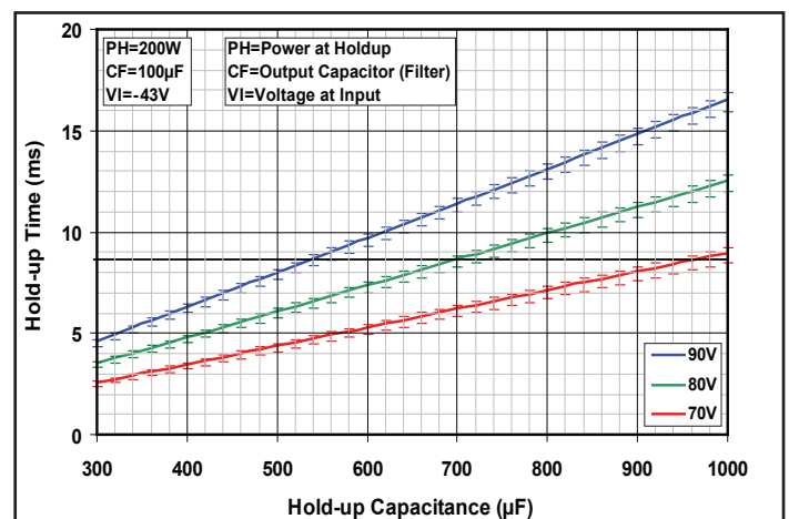
Figure E: Hold-up Time (ms) vs. Hold-up Capacitance (µF) at Hold-up Charge Voltages of 70V, 80V, and 90V (see Equation A). The AdvancedTCA hold-up time requirement is at most 8.70ms (solid horizontal line). The capacitor tolerance is not factored into this result. Error bars indicate the worst case range of hold-up time for a given hold-up capacitance.
