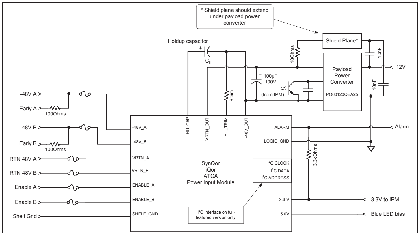
Figure H: Application Diagram
