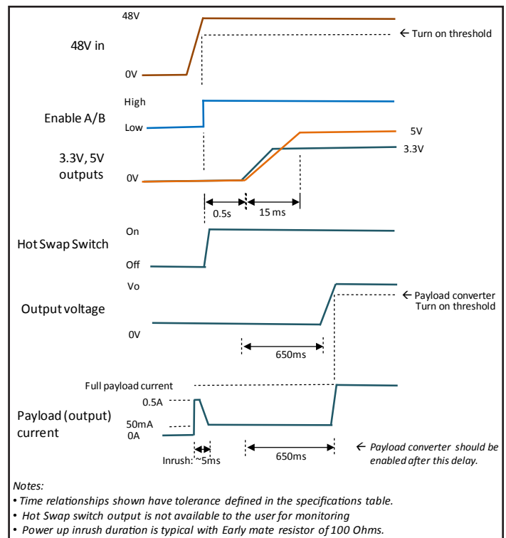
Figure D: Power up (Board insertion) timing diagram
