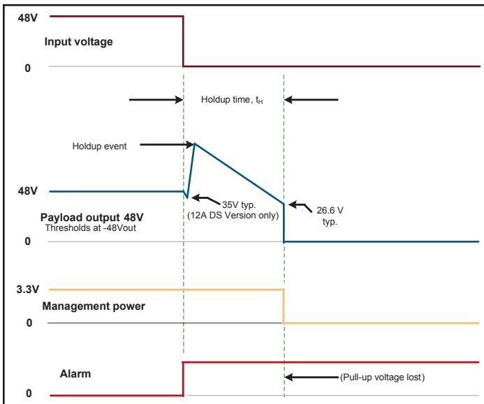
Figure B: Sudden Loss of Input Power
