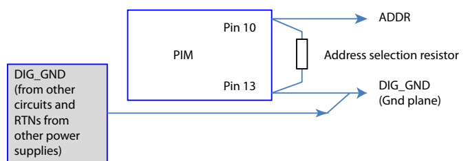
Figure J: Resistor Diagram
