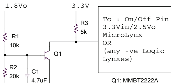
Fig. 4 Turn-on Interface Circuit for 1.8Vo to 2.5Vo MicroLynx (or any -ve LOGIC Devices).
