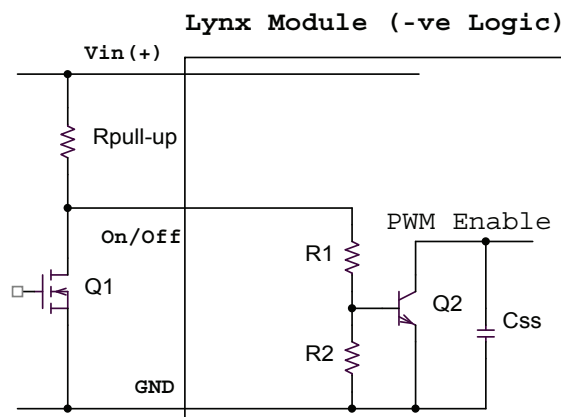
Fig. 2 Circuit configuration for using Negative Logic On/Off
