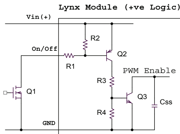
Fig. 1 Circuit configuration for using Positive Logic
