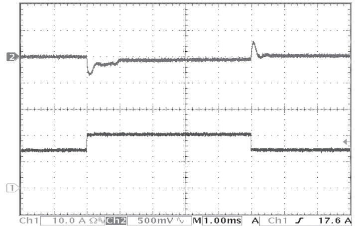
Figure 10: Output voltage response to step-change in load current (50%-75%-50% of I_{out(max)} ); dI/dt = 5A/\mu s . Load cap: 470 \mu F , 15 m \Omega ESR tantalum capacitor. Top trace: Vout (500mV/div), Bottom trace: Iout (10A/div).
