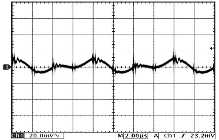
Figure 14: Output voltage ripple at nominal input voltage and rated load current (20 mV/div). Load capacitance: 1μF ceramic capacitor and 10μF tantalum capacitor. Bandwidth: 500 MHz. See Figure 11.
