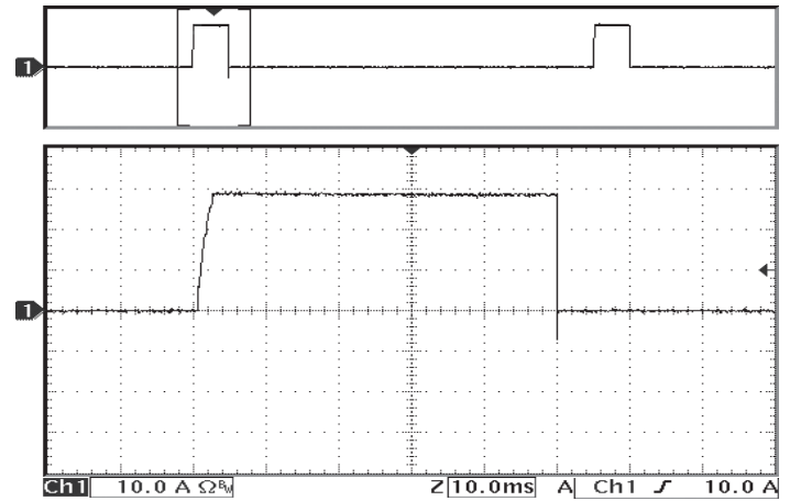
Figure 16: Load current (10A/div) as a function of time when the converter attempts to turn on into a 10 mΩ short circuit. Bottom trace (10ms/div) is an expansion of the on-time portion of the top trace (100ms/div).
