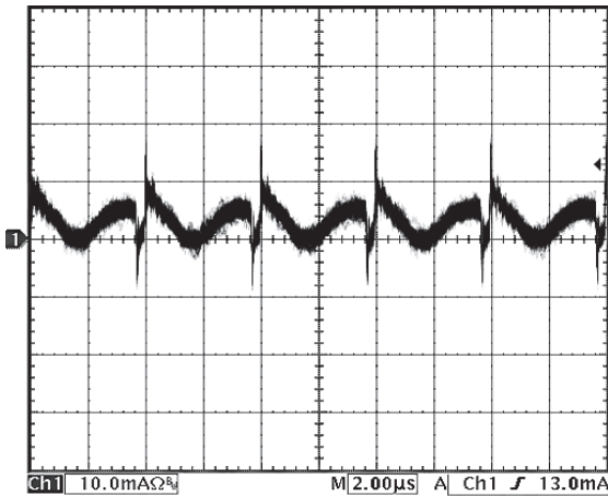
Figure 13: Input reflected ripple current, is, through a 4.7μH source inductor, using a 100μF input capacitor, at nominal input voltage and rated load current (10 mA/div). See Figure 11.
