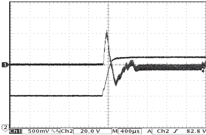
Figure 15: Output voltage response to step-change in input voltage (50V to 100V in 200μs). Load cap: 470μF, 15 mΩ ESR tantalum capacitor. Ch 1: Vout (500mV/div), Ch 2: Vin (20V/div), at zero load current.
