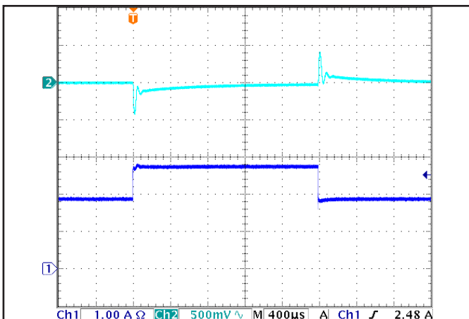
Figure 11: 3.3Vout response to a step-change in load current (50%-75%-50% of Iout(max): dI/dt = 1A/\mu s ). Load capacitance: 10uF ceramic capacitor. Top trace: 3.3Vout (500mV/div). Bottom trace: Iout (1A/div).
