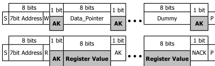
Figure I: Typical I 2 C read transmission. Note: S = START, W = WRITE, R = READ, AK = acknowledged, NACK = NOT acknowledged, P = STOP. Clear boxes originate in the I 2 C Master and shaded boxes originate in the I 2 C Slave.
