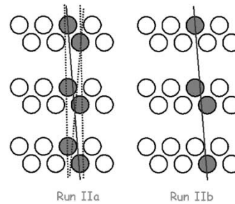
Fig. 3. The doublet (left) and singlet (right) schemes for CCT triggers. The circles represent three doublet layers of axial fibers in the CTT (not to scale). The solid line represents the actual track trajectory and the dark circles show which fibers are validated in each scheme. The dashed lines show the range of possible trajectories consistent with the validated fibers for the doublet scheme.
