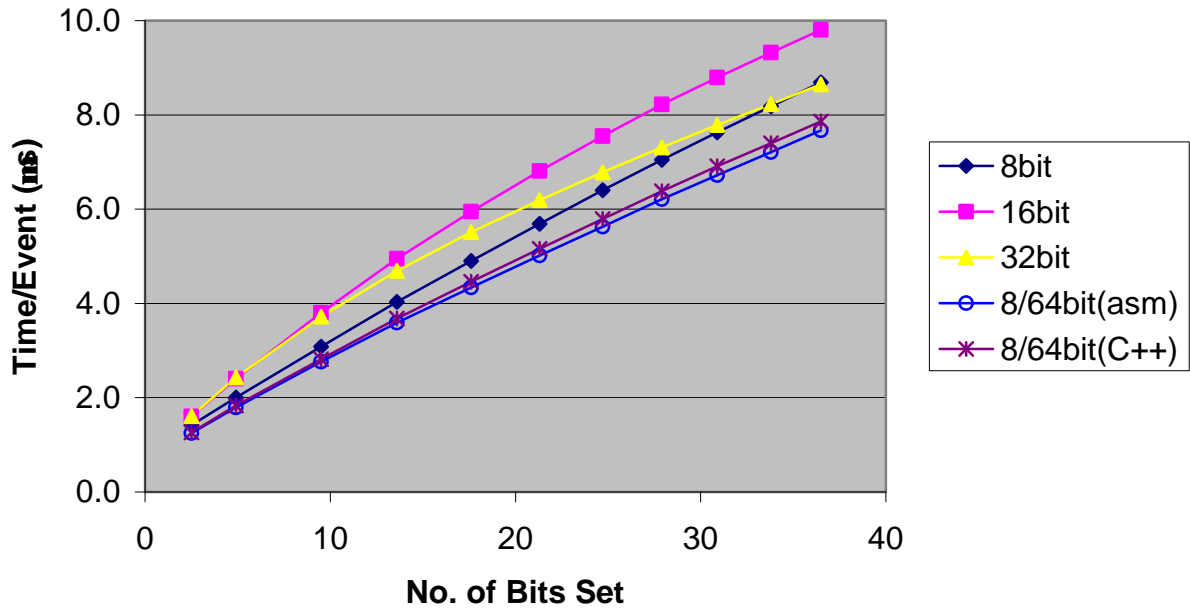
Event Time vs. Number of Bits for Different Search Block Sizes
