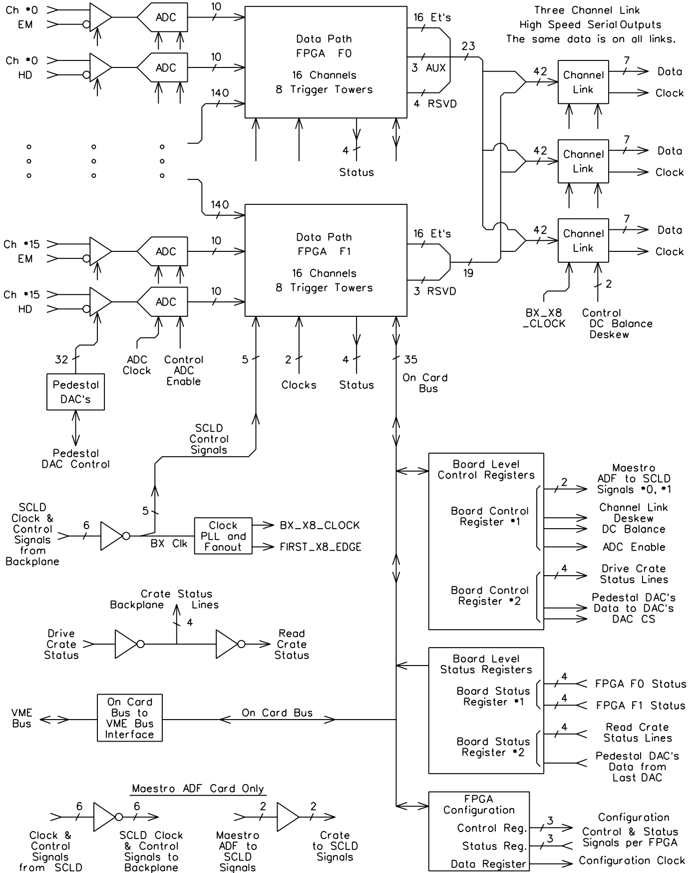
ADF-2 Card Block Diagram
