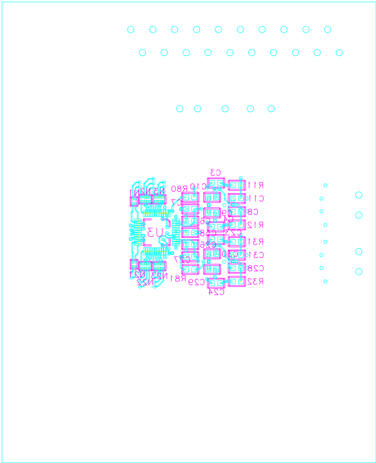
Layer #4 Solder
