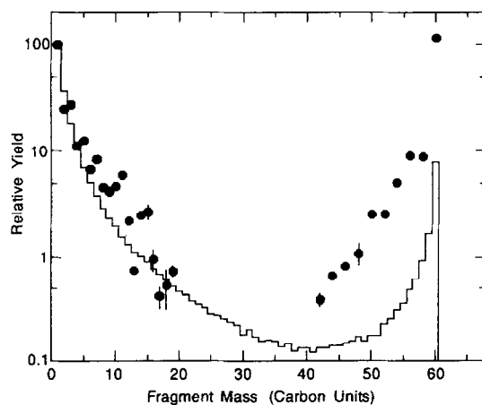
Fig. 4. Measured mass distribution (solid points) for positive fragments arising from C_{60} bombarded by 625-MeV ^{136}\text{Xe}^{35+} ions. The histogram is the distribution calculated on the basis of a percolation-multifragmentation model [7].
