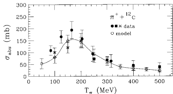
Fig. 2. Pion absorption cross section as a function of beam energy in \pi^+ + {}^{12}\text{C} scatterings. The data are taken from Refs. [19–21] (see text).
