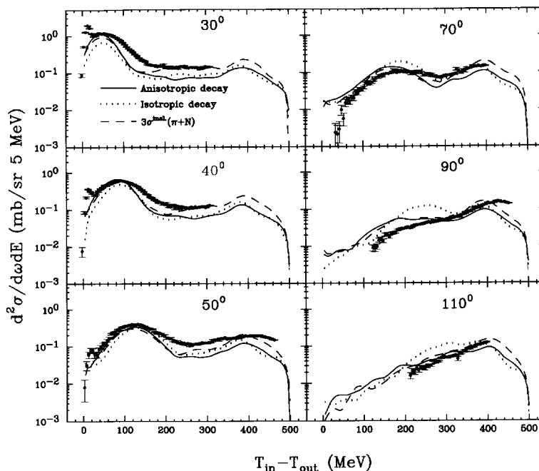
Fig. 3. Inclusive double differential cross sections of pions as a function of the pion laboratory angle and the pion energy loss, T_{in} - T_{out} , in 500 MeV C(\pi^+, \pi^+) reactions. The data (circles) are from Ref. [2].
