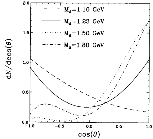
Fig. 1. The angular distribution of pions from the decay of \Delta^{++} resonance in its rest frame.
