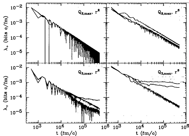
FIG. 3. Positive Lyapunov exponents for the single-particle trajectories resulting from a time evolution in an external static multipole deformed potential with deformation equal to the maximum deformation obtained in the self-consistent calculations of Fig. 2.
