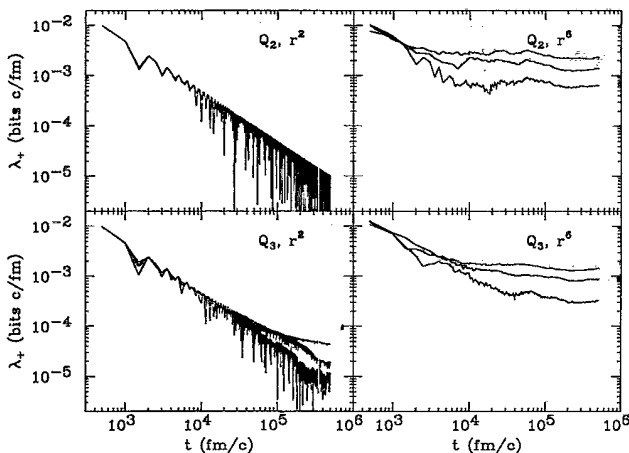
FIG. 2. Positive Lyapunov exponents for the single-particle trajectories leading to the time evolution of the collective multipole moments shown in Fig. 1.
