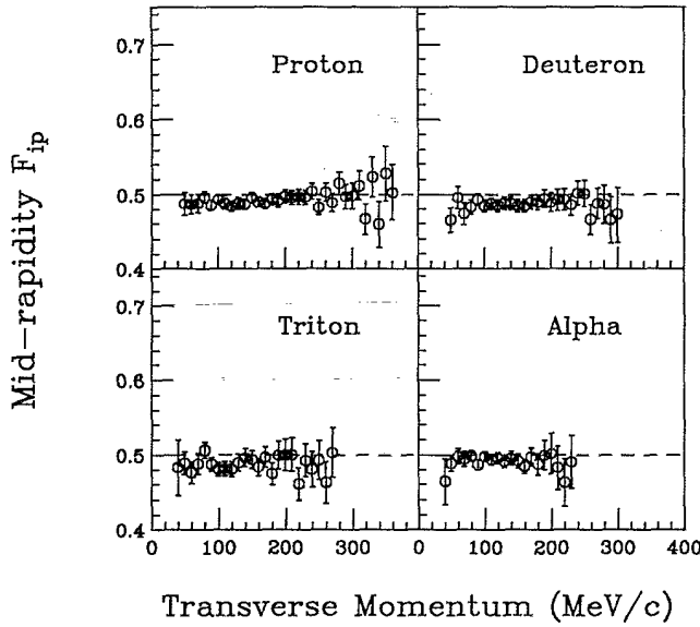
FIG. 13. Anisotropy fractions for 100 MeV/nucleon Ar+V data as function of p^\perp /nucleon. The rapidity of the particles was restricted to y_{c.m.} \pm .02 for this figure.
