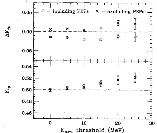
FIG. 20. Final BUU anisotropy fractions calculated with and without including nucleons emitted in the first 60 fm/c (PEP's).
