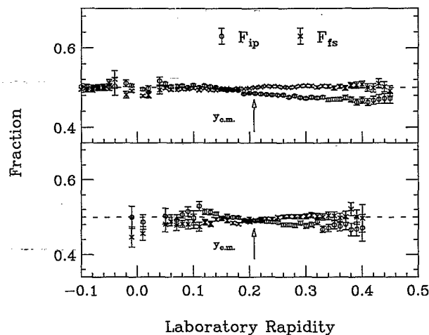
FIG. 12. Anisotropy fractions as function of rapidity for 100 MeV/nucleon Ar+V data.
