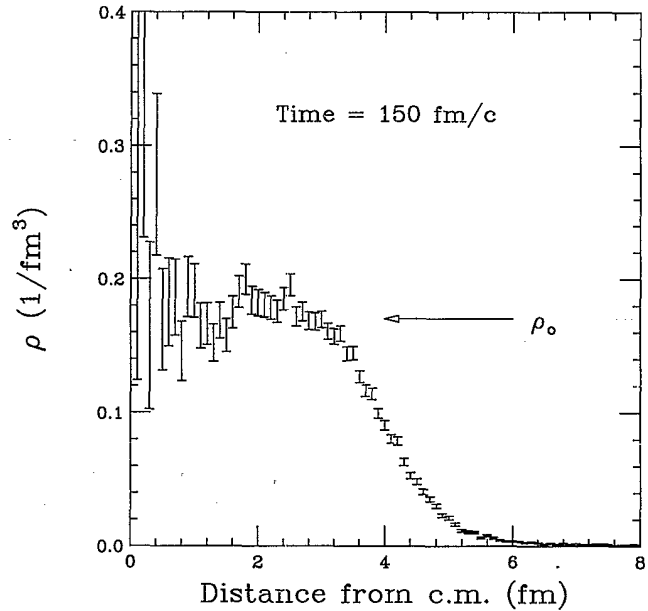
FIG. 16. Number density of nucleons as a function of distance from the center of mass in coordinate space at t=150 fm/c for one BUU calculation. The error bars in this figure are taken from the square root of the number of counts. Normal nuclear matter density is indicated by the arrow.
