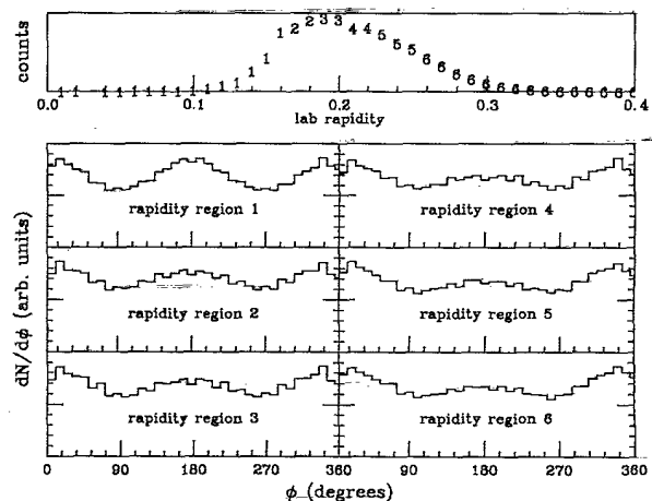
FIG. 8. Azimuthal distributions of helium produced in 35 MeV/nucleon Ar+V collisions divided into six rapidity bins.
