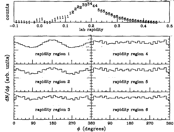
FIG. 7. Azimuthal distributions of hydrogen produced in 35 MeV/nucleon Ar+V collisions divided into six rapidity bins.
