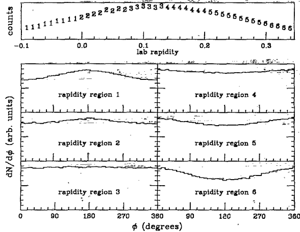
FIG. 2. Azimuthal distributions with respect to the reaction plane for a simulated source with transverse momentum flow.
