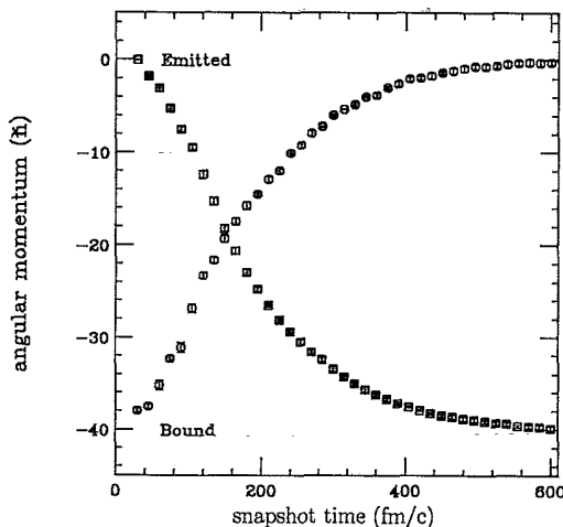
FIG. 19. Angular momentum in the BUU calculation as a function of time.
