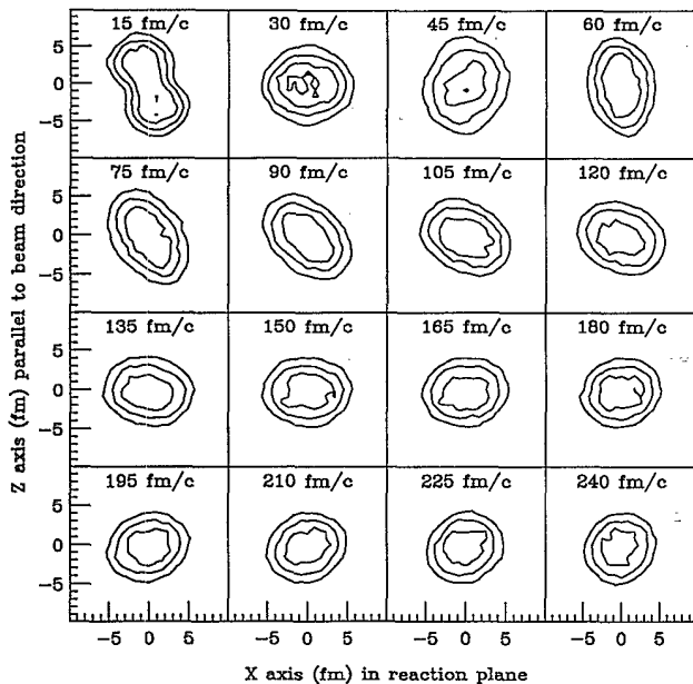
FIG. 15. BUU coordinate space density distribution projected on to the x - z plane. The projectile begins on the lower right-hand region in the 15 fm/c snapshot, offset in the positive x direction by convention.
