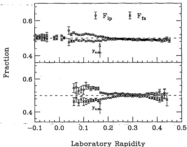
FIG. 11. Anisotropy fractions as function of rapidity for 65 MeV/nucleon Ar+V data.
