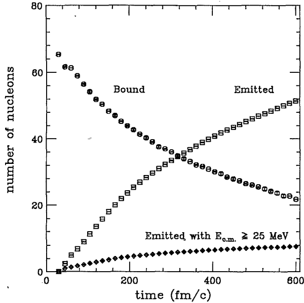
FIG. 18. The number of nucleons in the residue (circles) and the number of nucleons emitted (squares) are shown as a function of time for the BUU calculation. Those emitted with a center-of-momentum energy greater than 25 MeV are denoted by diamonds.
