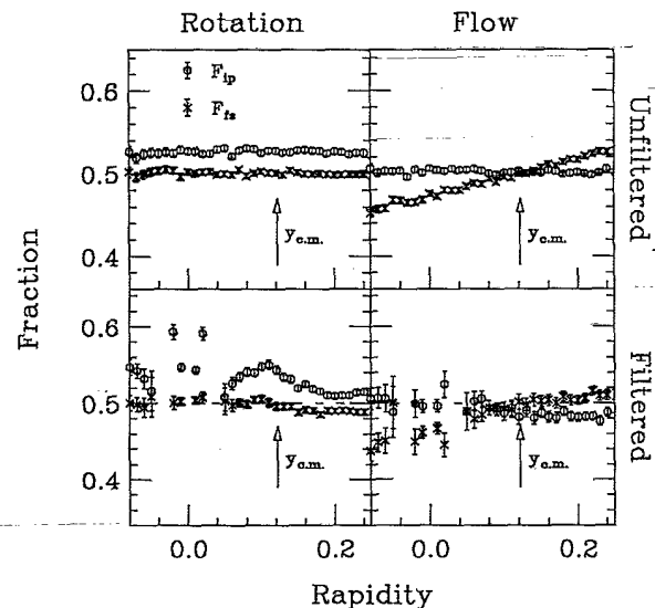
FIG. 4. Anisotropy fractions for a oblate momentum distribution simulating rotation (left panels) and a prolate distribution with transverse momentum flow (right panels). The simulations are shown before (top panels) and after (bottom panels) being passed through a software representation of the acceptance of the 4\pi Array. The dashed line represents the fractional value expected if the azimuthal distributions are isotropic.
