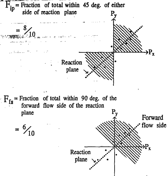
FIG. 3. Geometrical definition of the anisotropy parameters F_{ip} and F_{fs} projected onto the p_x - p_y plane.
