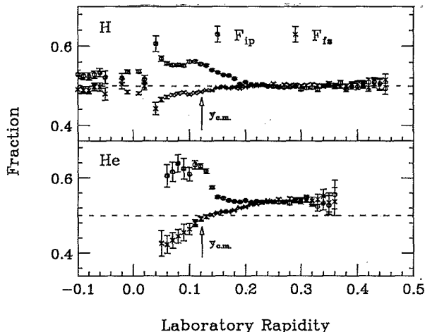
FIG. 6. Anisotropy fractions as function of rapidity for 35 MeV/nucleon Ar+V data.
