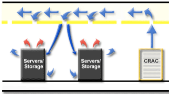
Figure 2. Overhead distribution system.
