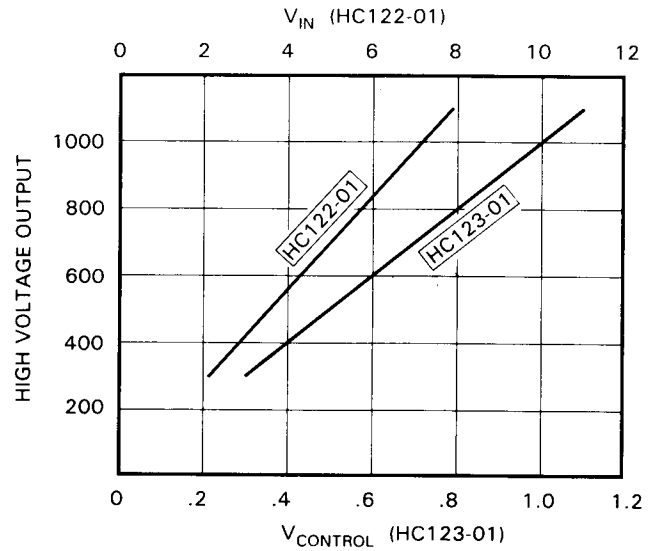
Figure 3. High voltage output vs. input
