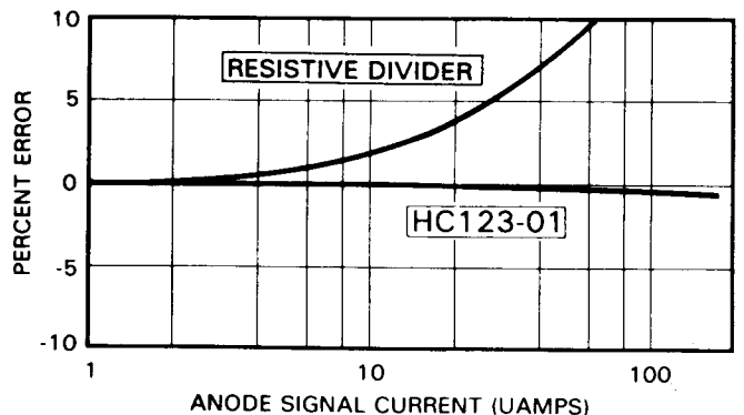
Figure 4. DC linearity
