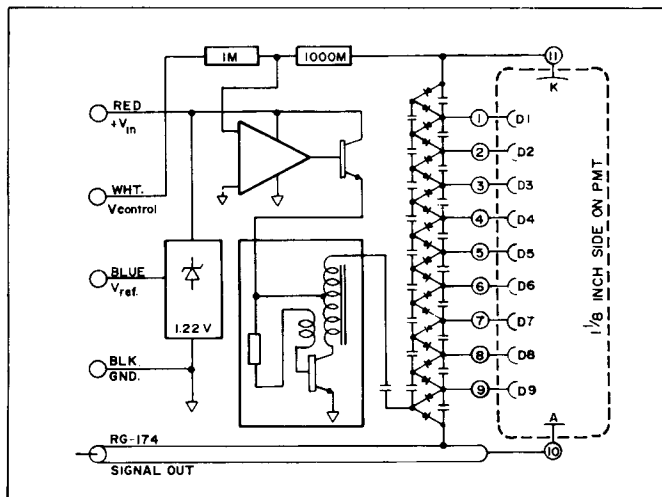
Figure 2. HC123-01 schematic diagram
