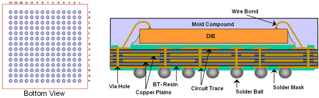
Figure 2 • Bottom View and Cross-Section of Four-Layer CSPs
