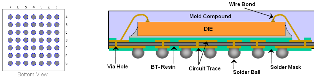
Figure 1 • Bottom View and Cross-Section of Two-Layer CSPs
