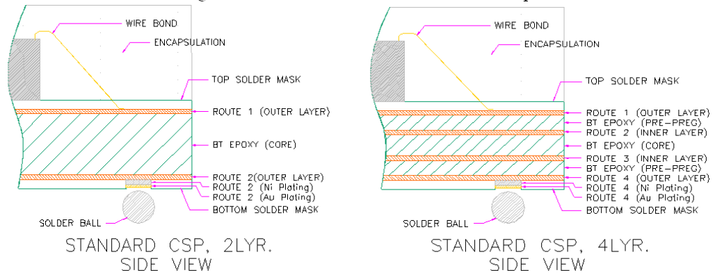
Figure 3 • Detail of Substrate Stack-Up Construction
