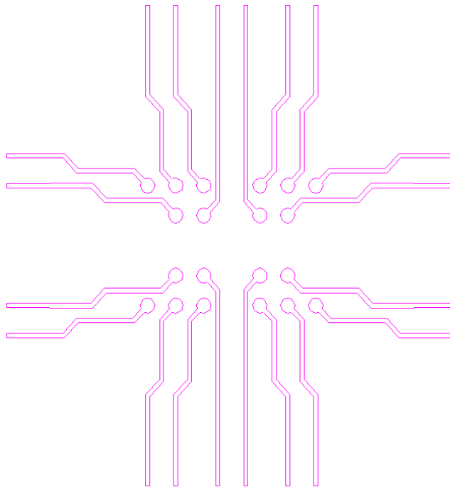
Figure 19 • Suggested Board Layout of Soldered Pads for CS196 CSPs (PCB Lower Layer)
