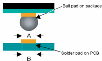
Figure 4 • Pad Design Recommendations
