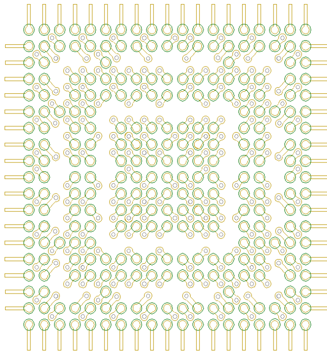
Figure 23 • Suggested Board Layout for NSMD, Line Width 0.1 mm, of Soldered Pads for CS281 CSPs (PCB Top Layer)
