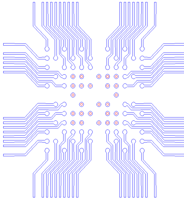
Figure 25 • Suggested Board Layout of Soldered Pads for CS281 CSPs (PCB Lower Layer)
