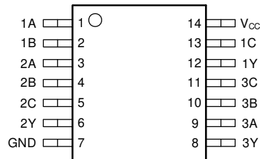
Figure 4-1. SN74LV10A . . . D, NS, OR PW PACKAGE (TOP VIEW)
