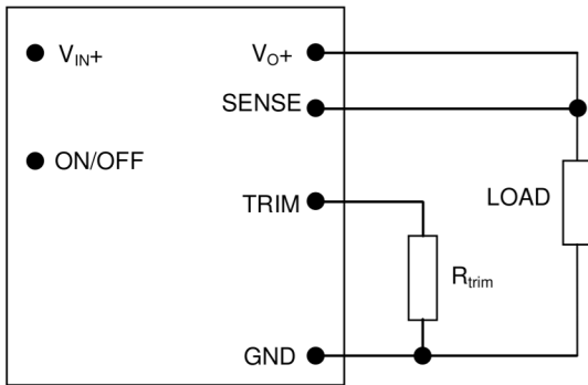
Figure 40. Circuit configuration for programming output voltage using an external resistor.
