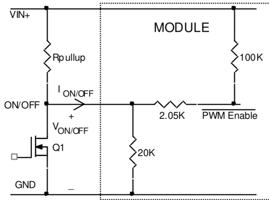
Figure 38. Circuit configuration for using negative On/Off logic.
