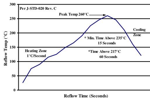
Figure 46. Recommended linear reflow profile using Sn/Ag/Cu solder.
