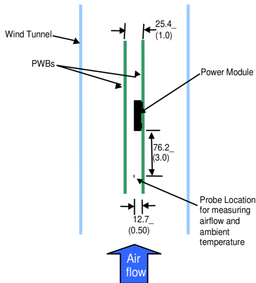
Figure 44. Thermal Test Setup.
