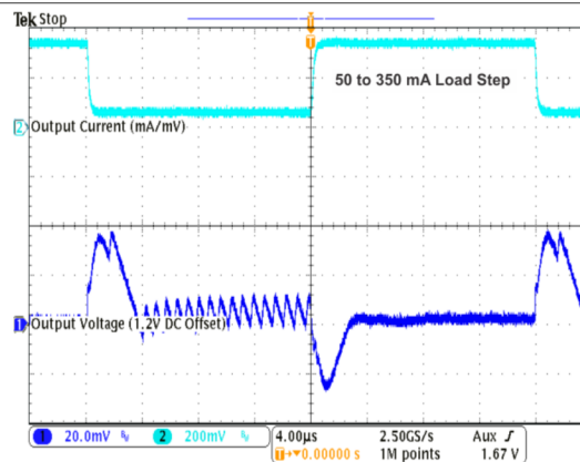
Figure 34. Load Transient Response in PFM/PWM Operation
