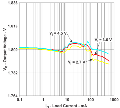
V_O = 1.8\text{ V} PFM/PWM Operation (TPS82671)
