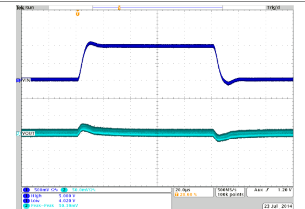
Figure 37. Line Transient Response for TPS8268105 (Vout = 1.05V; Iout = 900mA, Vin = 4V to 5V to 4V)
