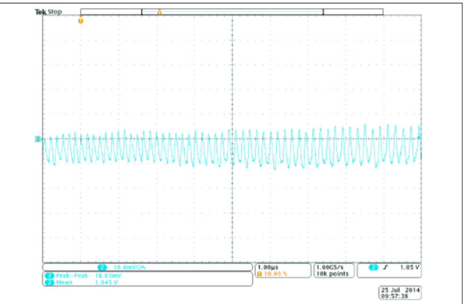
Figure 39. Output Voltage Ripple for TPS8268105 (Vin = 5V, Vout = 1.05V, Iout = 900mA)
