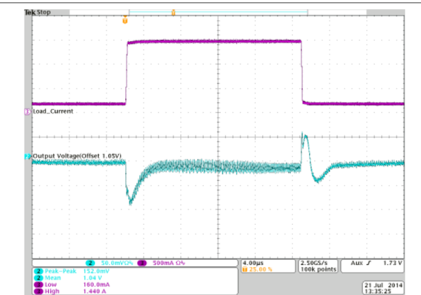
Figure 36. Load Transient Response for TPS8268105 (Vout = 1.05V, Iout = 160mA to 1.44A to 160mA, Vin = 5V)
