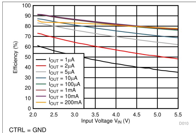
Figure 8. TPS82740A Efficiency V_{OUT} = 1.8V
