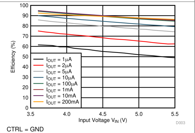
Figure 9. TPS82740A Efficiency V_{OUT} = 2.1V
