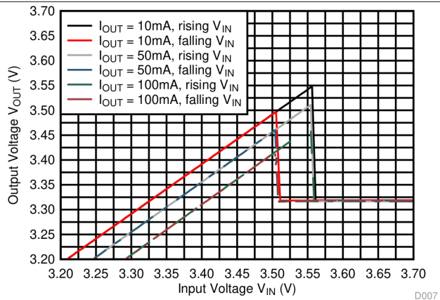
Figure 21. TPS82740B 100% Mode Transition V_{OUT} = 3.3V
