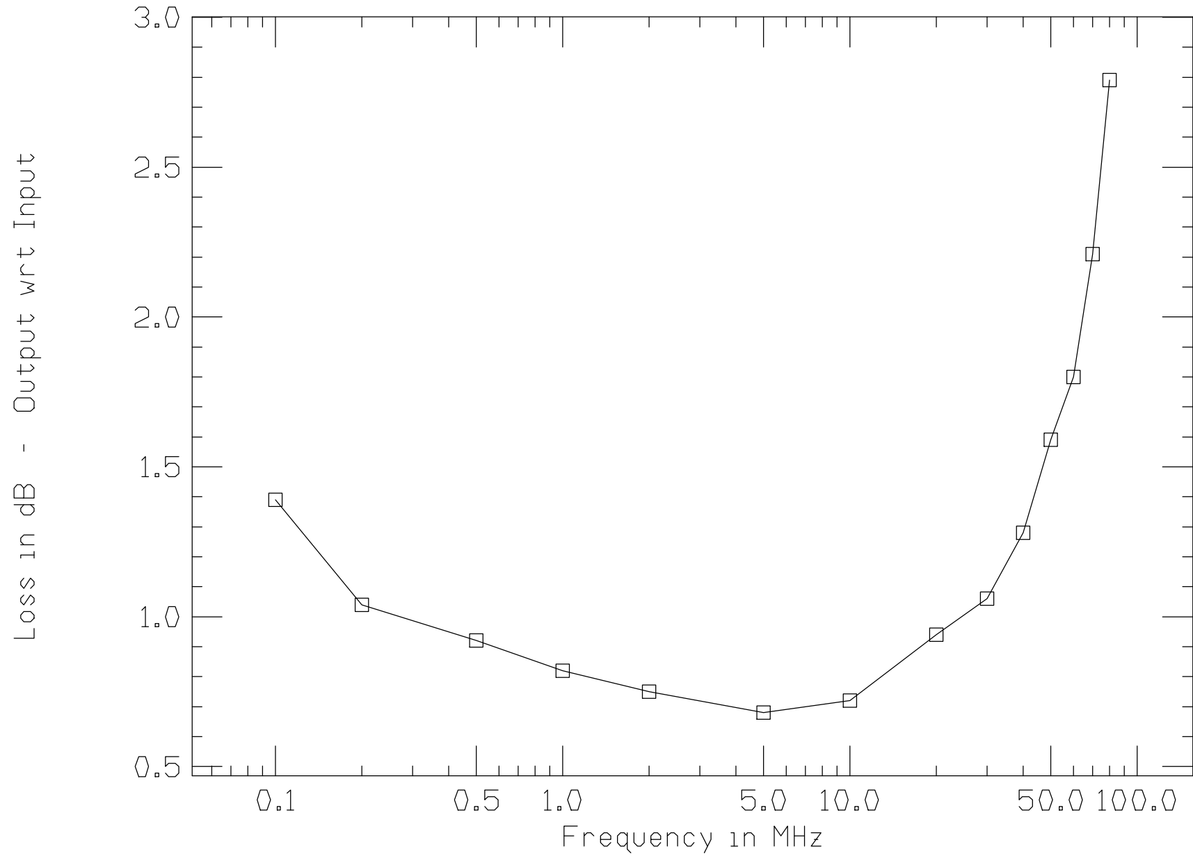
Murata 78602/4JC 1:1:1 Transformer 5-Mar-2023
