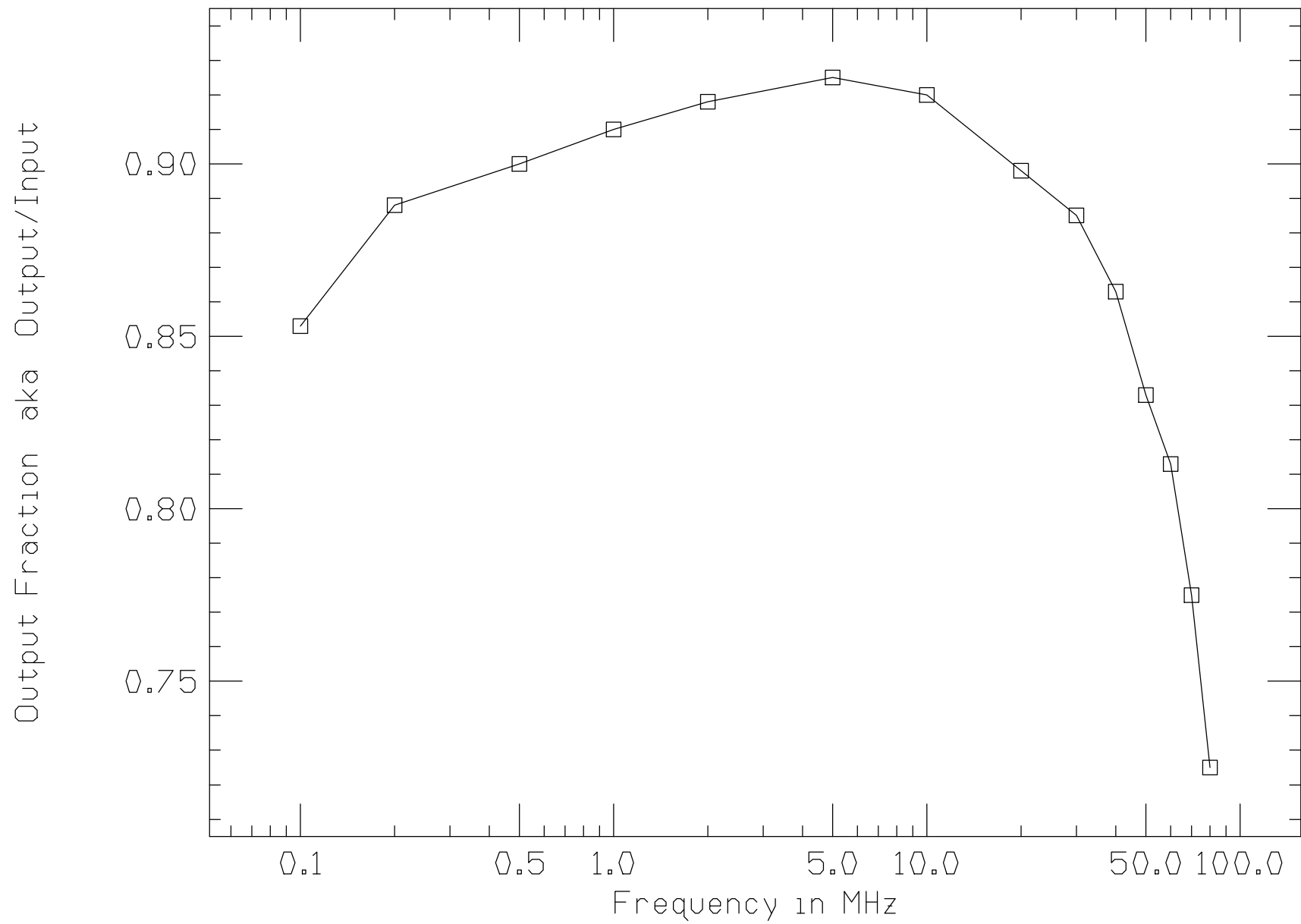
Murata 78602/4JC 1:1:1 Transformer 5-Mar-2023
