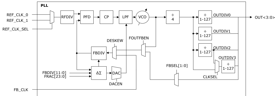
Figure 4-11. Frequency Synthesis
