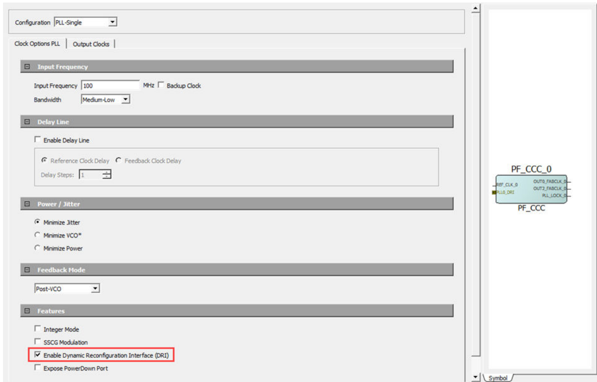
Figure 4-29. Clock Conditioning Circuitry Window
