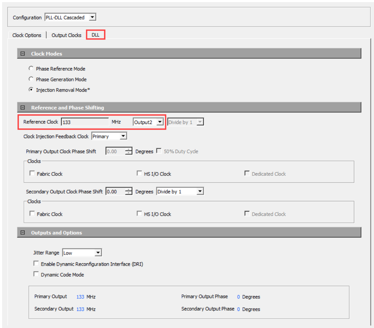
Figure 4-28. PLL-DLL Cascading
