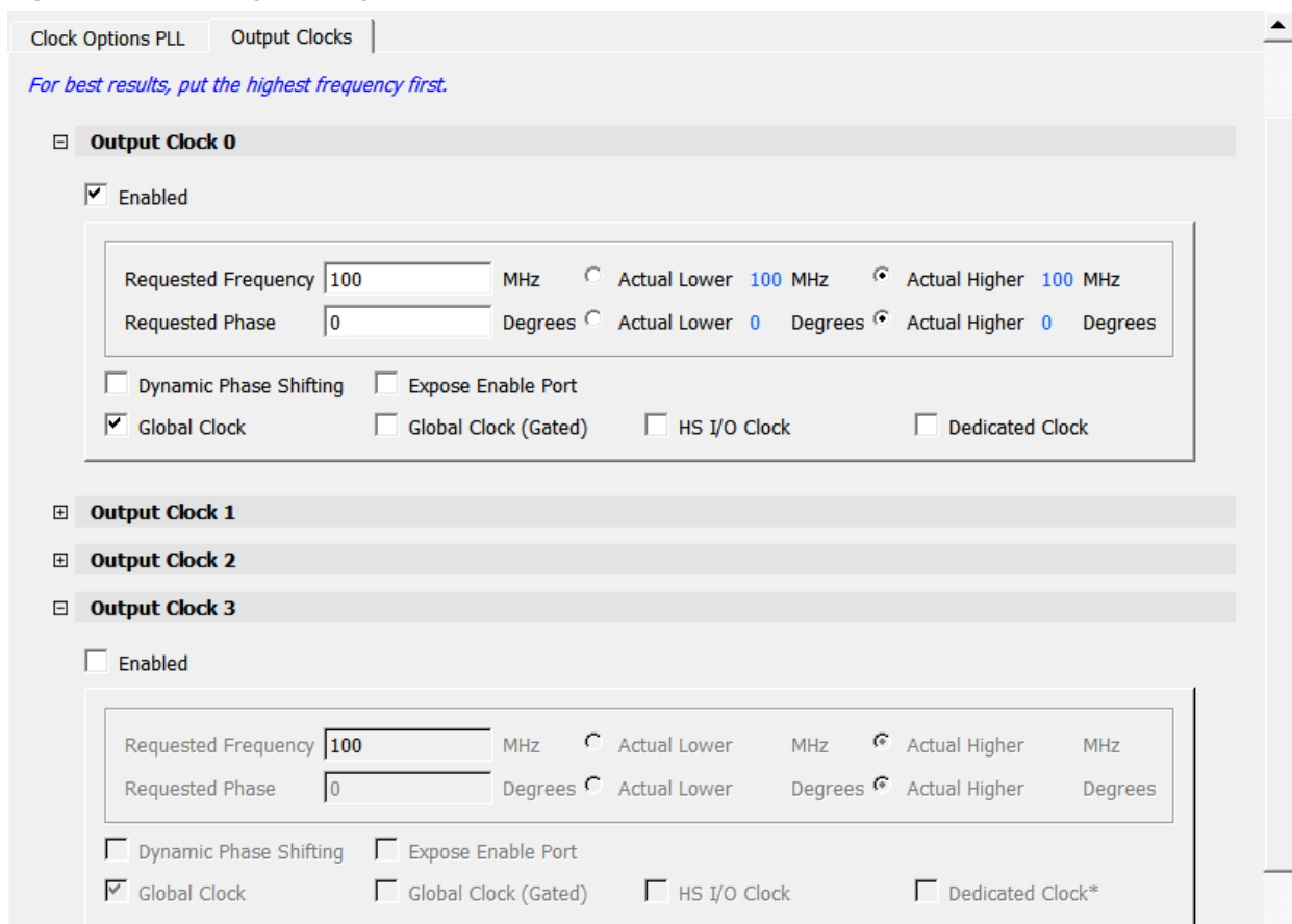
Figure 4-23. PLL-Single Configuration—Output Clocks
