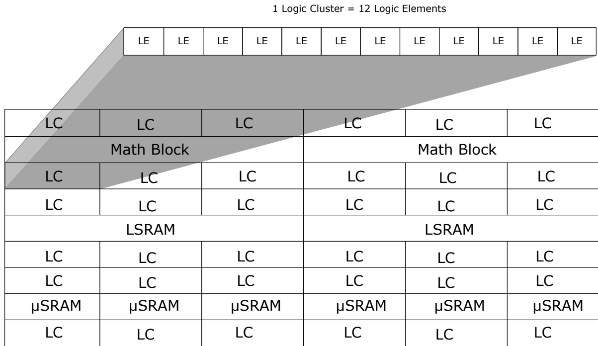
Figure 2-3. Sector Representation
