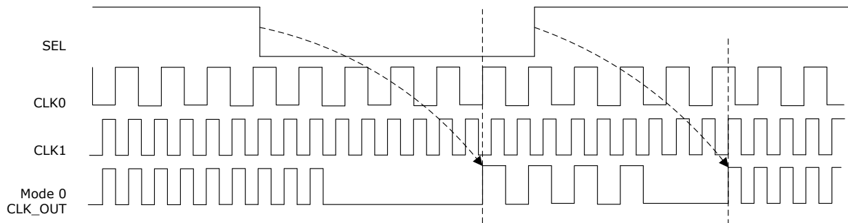
Figure 2-13. Mode 1: Clock Switching when Current Clock (CLK0) is not Active
