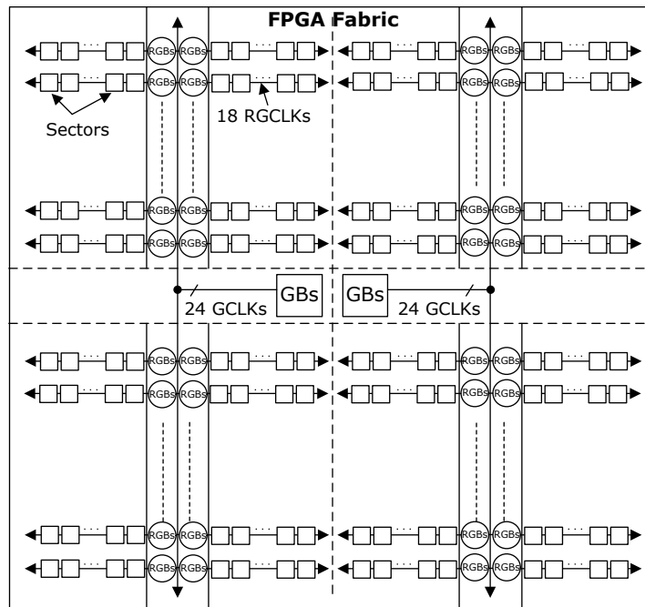
Figure 2-2. FPGA Fabric—Global Clock Routing Architecture
