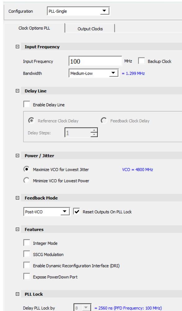
Figure 4-22. PLL-Single Configuration—Clock Options PLL
