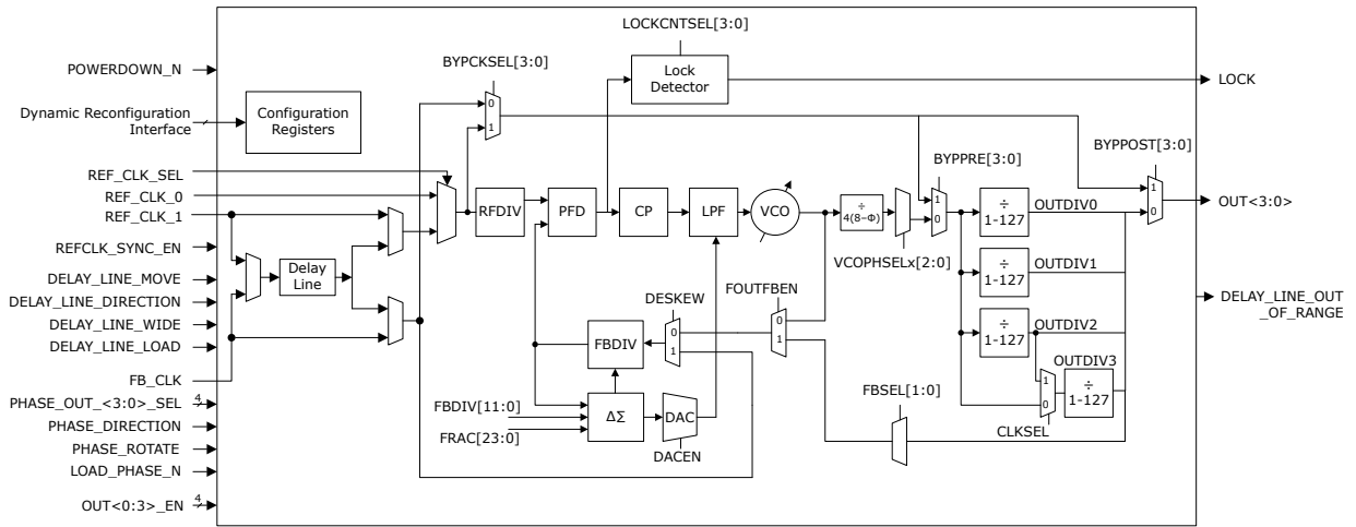
Figure 4-3. PLL Block Diagram
