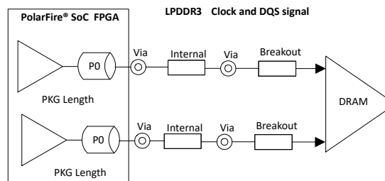
Figure 8-7. LPDDR3 Clock and DQS signal Routing
