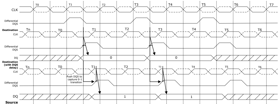
Figure 5-1. DQS Delay
