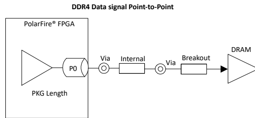
Figure 7-11. DDR4 Data Signal Point-to-Point
