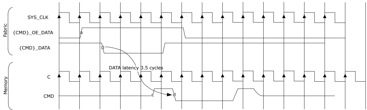
Figure 3-47. Command Timing
