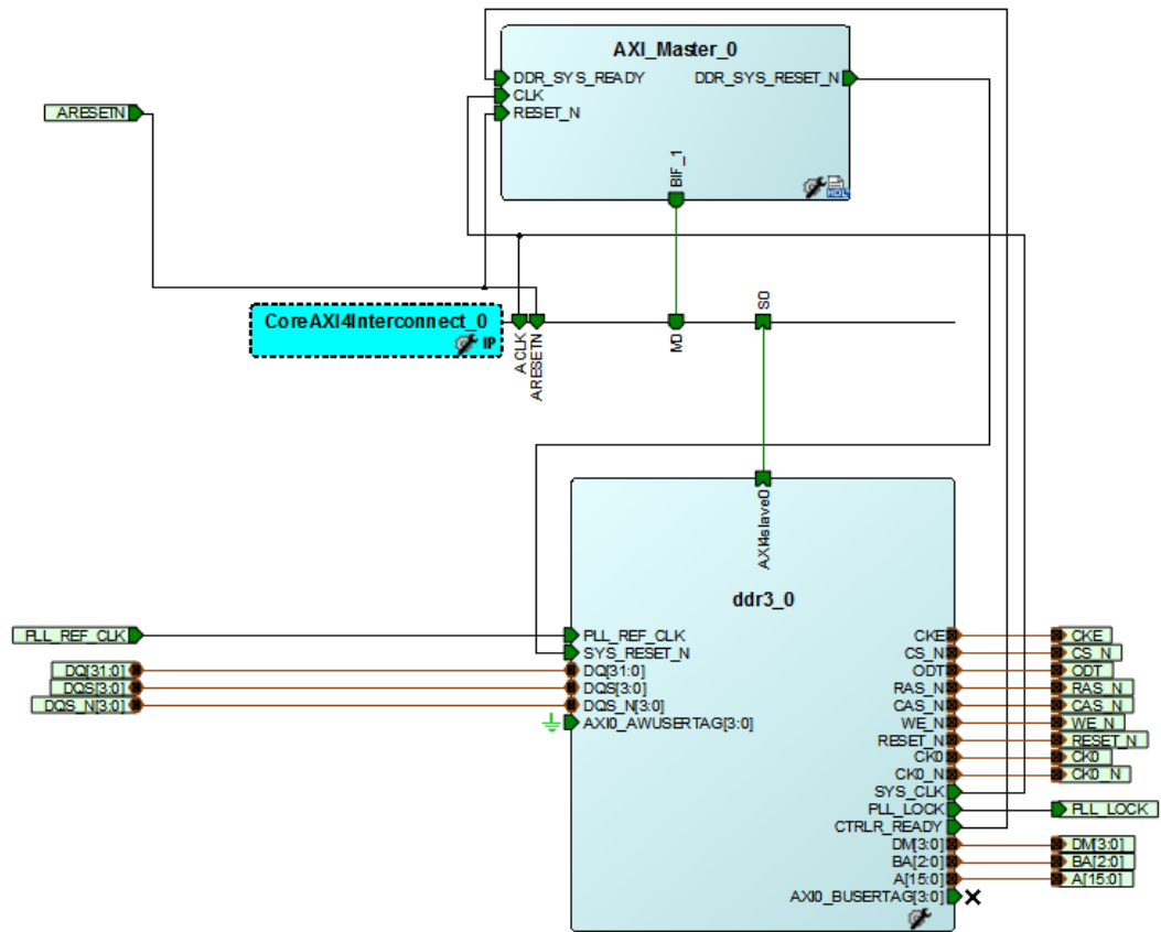
Figure 3-78. SmartDesign Connection—AXI
