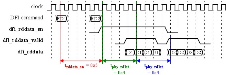
Figure 3-39. DFI Read Burst Example
