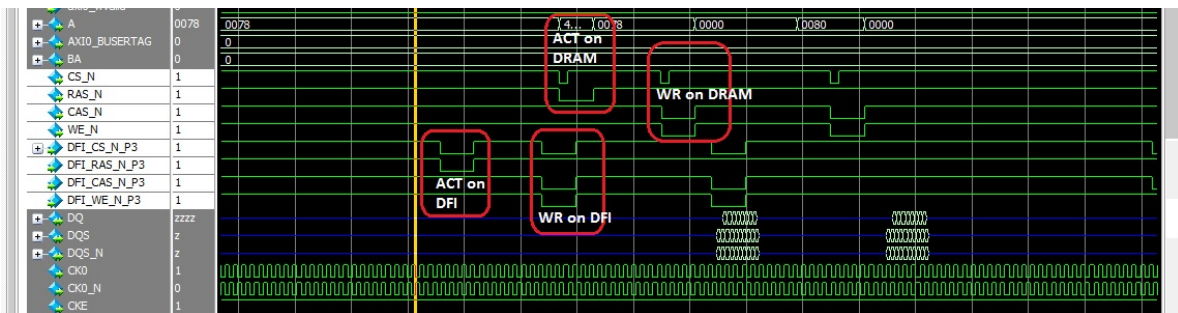
Figure 3-36. ACTIVATE AND WRITE COMMANDS ON DFI & DRAM (16BIT INTERFACE)
