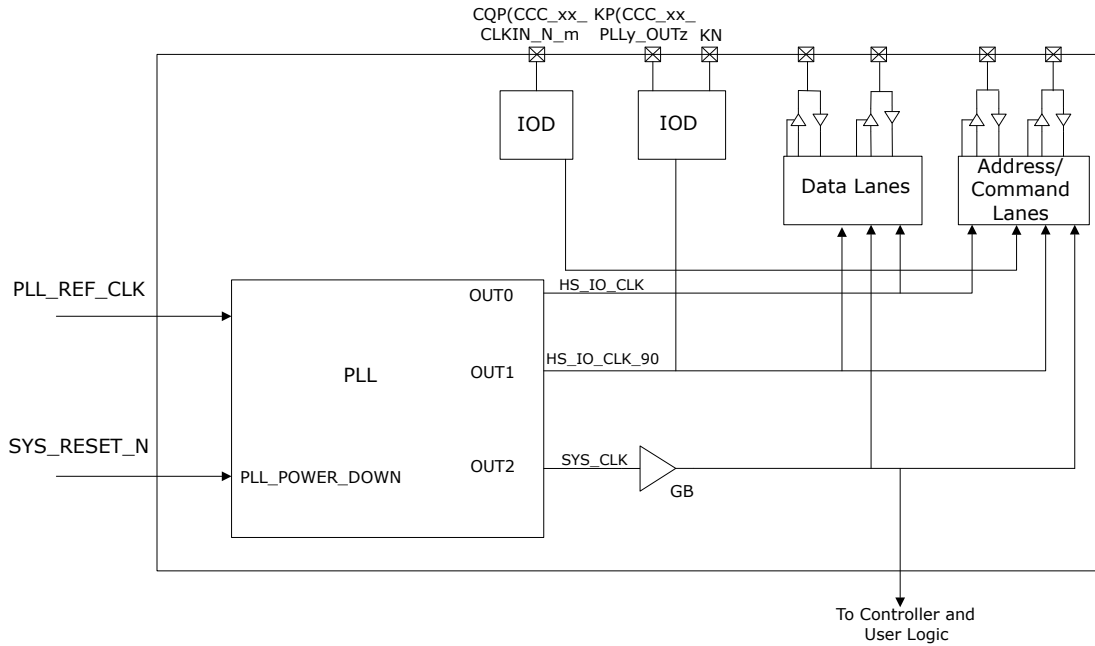
Figure 6-7. QDR Clocking Structure
