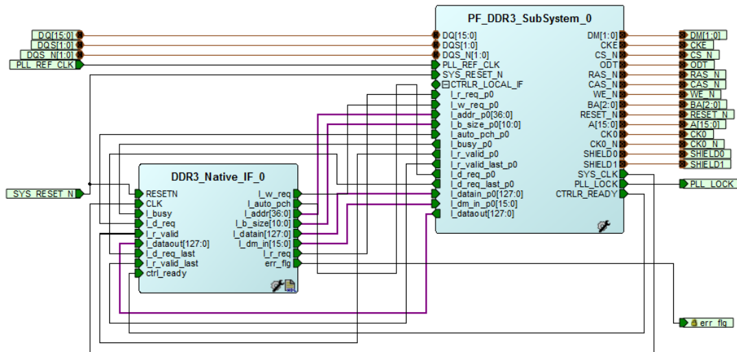
Figure 3-83. SmartDesign Connection—Native Interface
