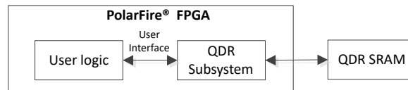
Figure 6-25. QDR Subsystem accessed through User Interface
