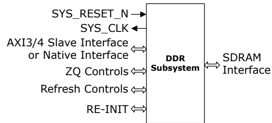
Figure 3-13. Fabric DDR Subsystem Ports
