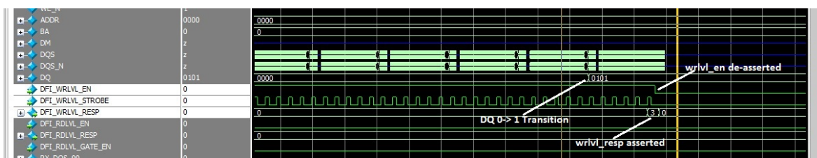
Figure 3-28. DFI Write Leveling Complete
