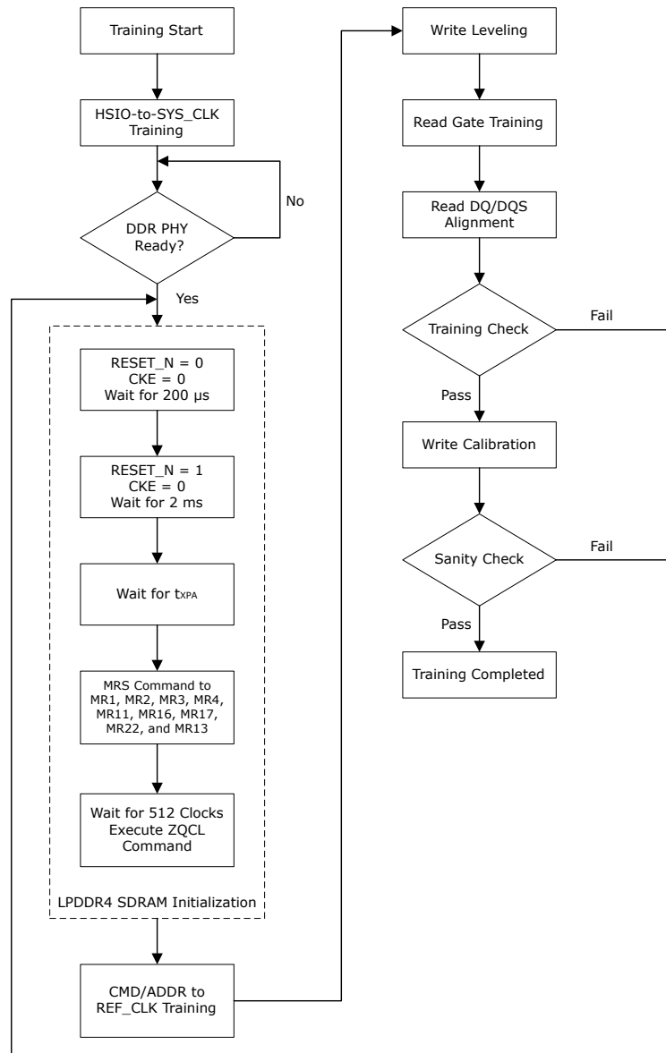
Figure 4-4. Automatic Initialization Flow for LPDDR4 Memory
