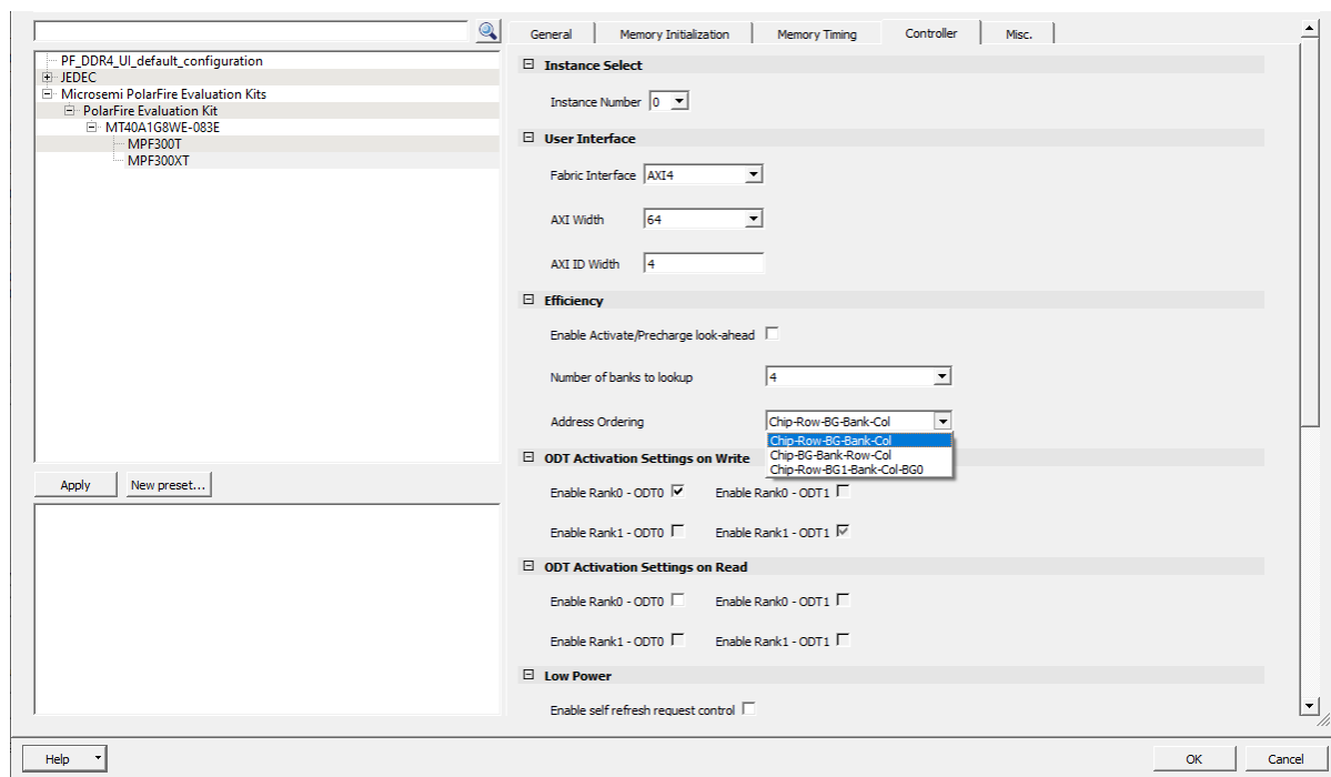
Figure 3-67. Address Ordering—Chip-Row-BG1-Bank-Col-BG0
