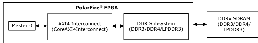
Figure 3-76. DDR Subsystem Accessed Through AXI4 Interface
