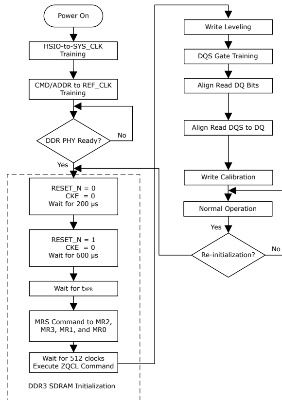
Figure 4-1. Automatic Initialization Flow for DDR3 Memory
