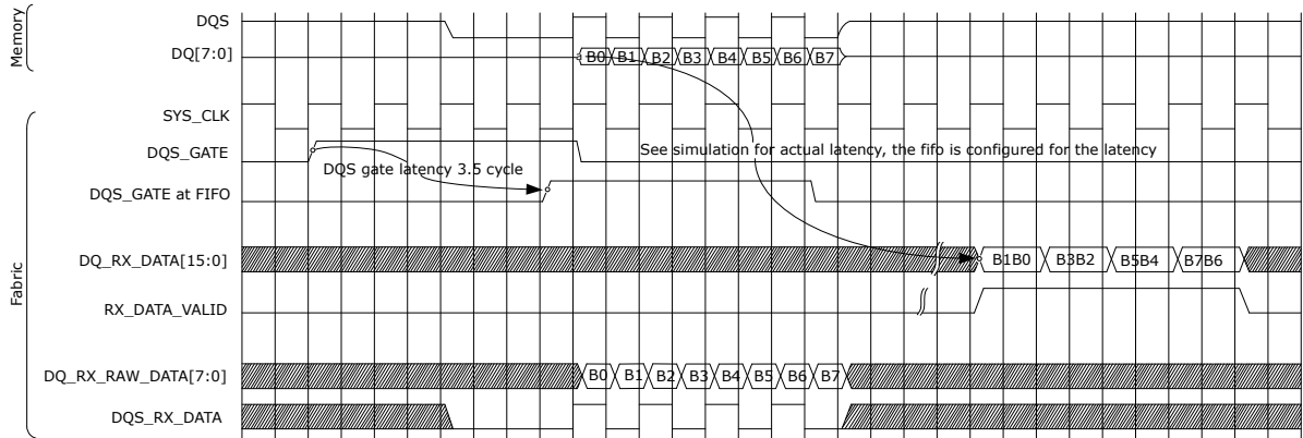
Figure 3-48. DQ/DQS Receive
