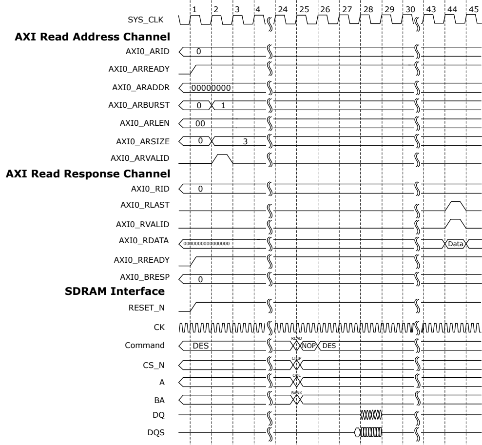
Figure 3-19. AXI Single Read Transaction
