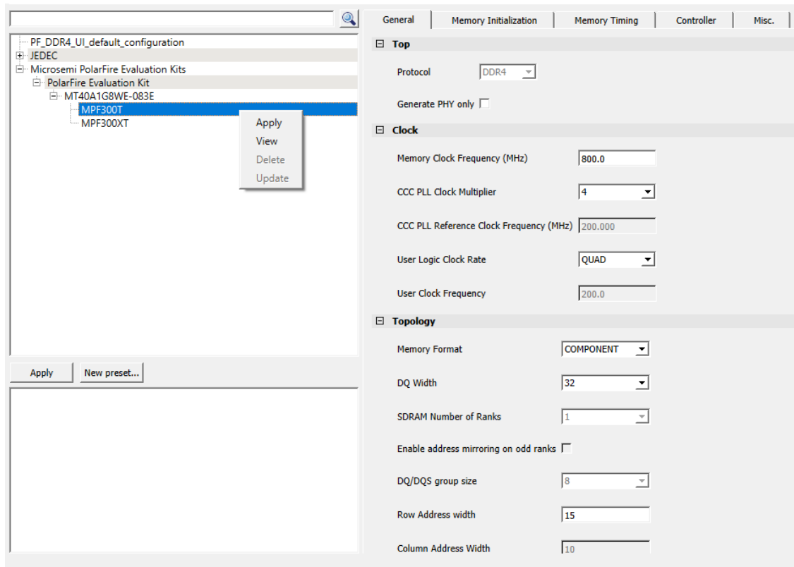
Figure 3-62. PF_DDR4 Configurator—Preset Configuration
