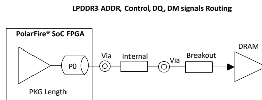
Figure 8-6. LPDDR3 Address/Control/DQ/DM Signal Routing
