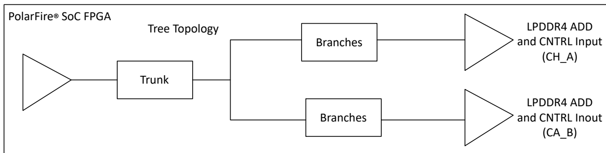
Figure 8-15. Dual-Channel LPDDR4 Interface Routing
