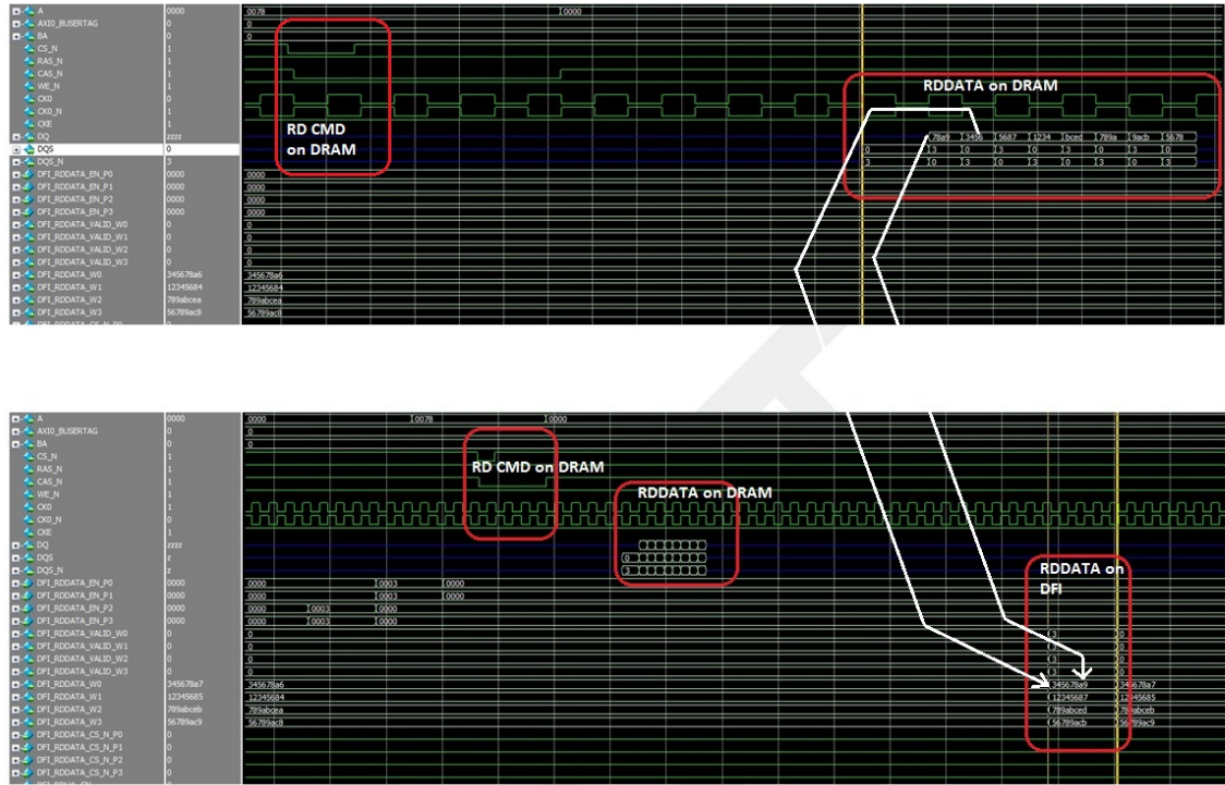
Figure 3-41. RDDATA ON DFI - 32 BIT BL8 ON DRAM TRANSLATE TO DFI 256 BITS (4 X 64)
