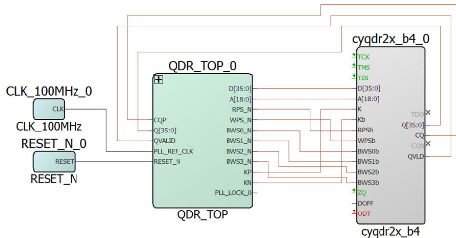
Figure 6-28. QDR SmartDesign Testbench
