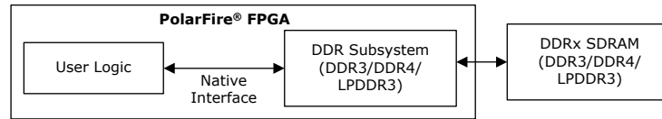
Figure 3-81. DDR Subsystem Accessed Through Native Interface
