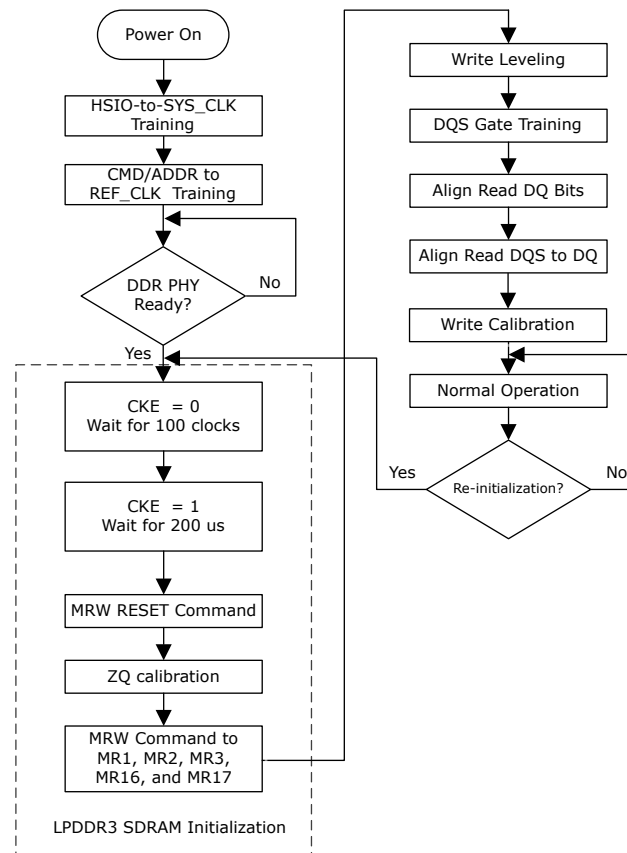
Figure 4-3. Automatic Initialization Flow for LPDDR3 Memory
