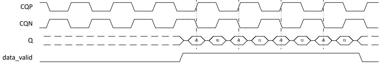
Figure 6-6. Data capture after moving CQP to center rising edge data
