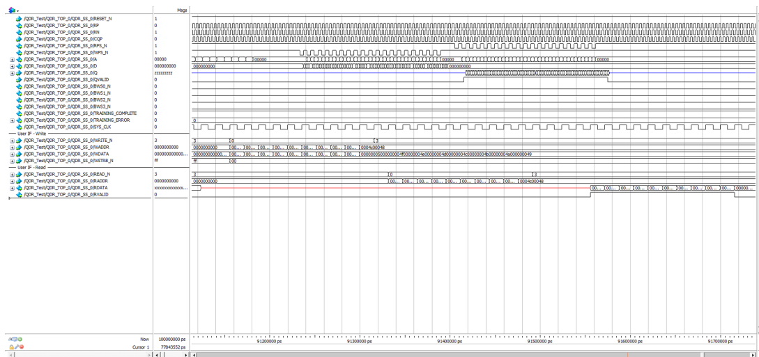
Figure 6-29. QDR Read and Write Transactions- RTL_FULL
