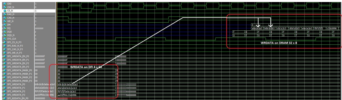
Figure 3-38. WRDATA ON DFI & DRAM - DFI 256 BITS (4 X 64) TRANSLATE TO 32 BIT BL8 ON DRAM
