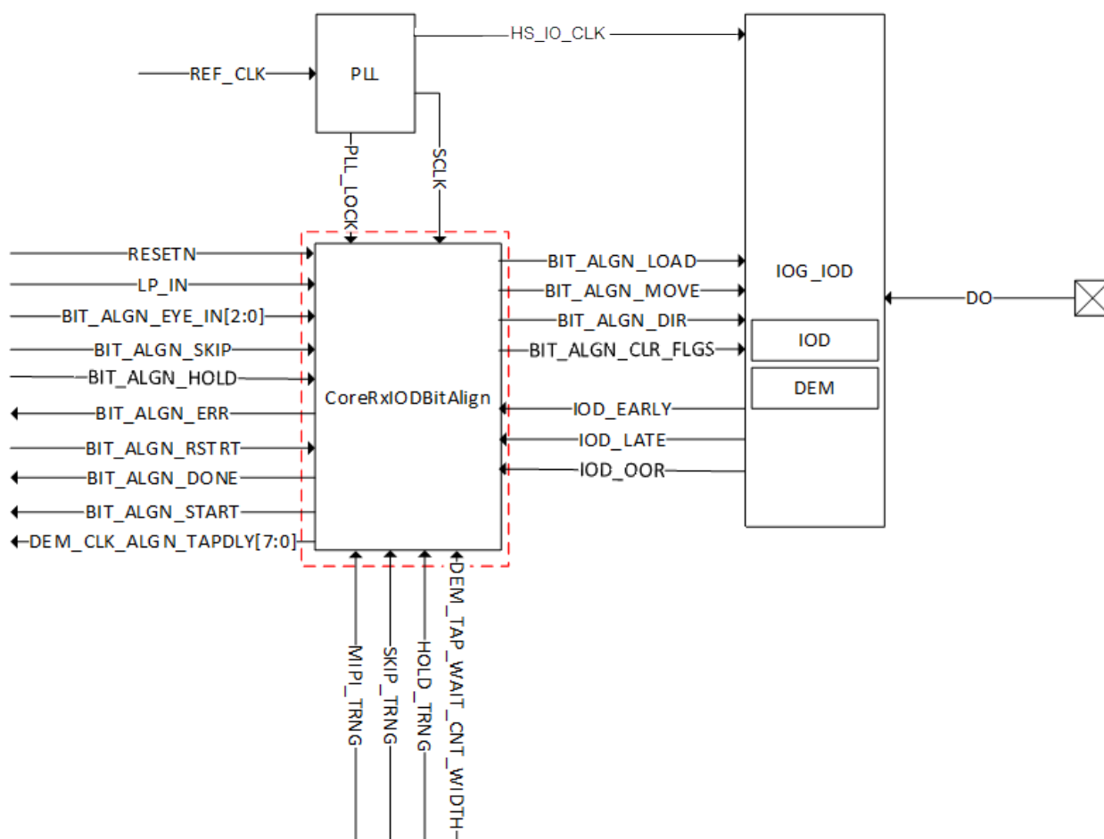
Figure 11-7. CoreRxIOBitAlign Implementation Diagram
