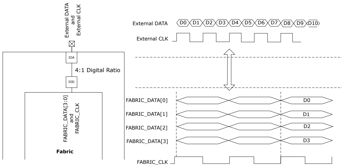
Figure 8-8. I/O Digital
