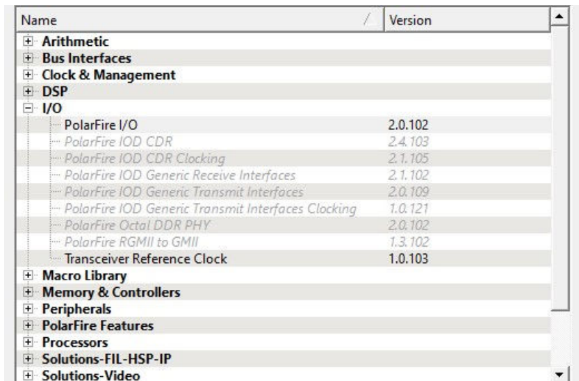
Figure 9-6. I/O Configurator
