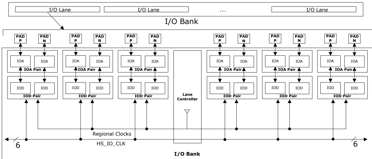
Figure 8-9. I/O Lanes
