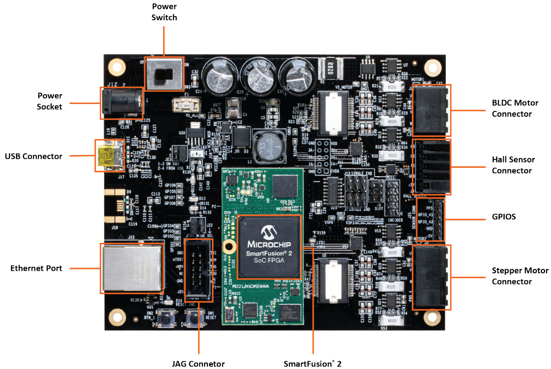
Figure 2-4. SmartFusion2 Motor Control Kit
