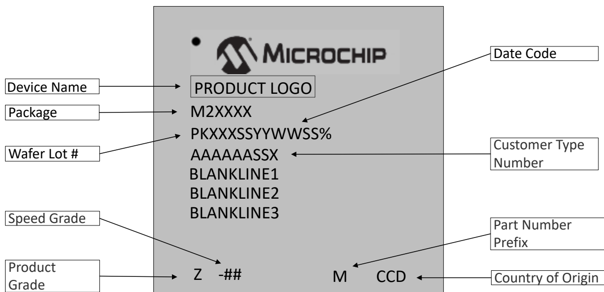
Figure 1-3. Marking Specifications
