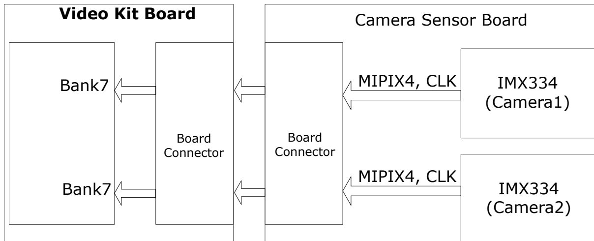
Figure 3-6. MIPI-RX Connection
