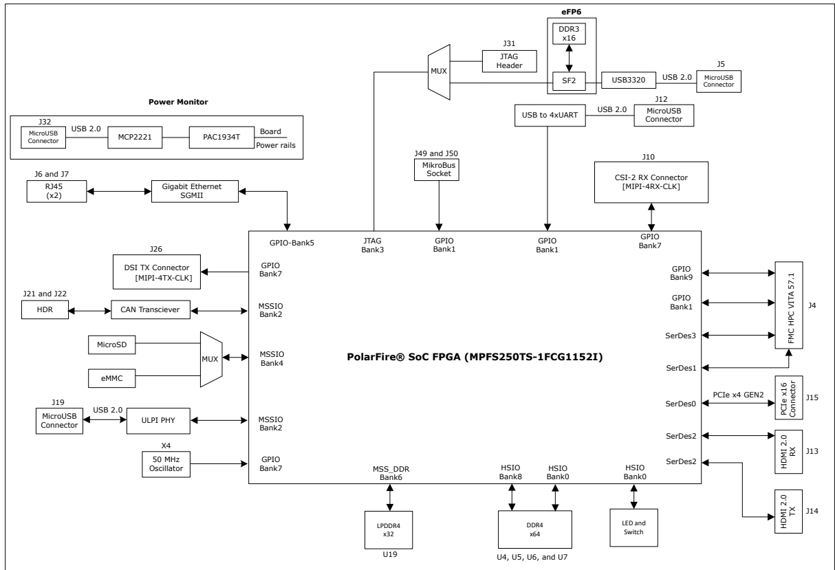
Figure 1-1. Block Diagram
