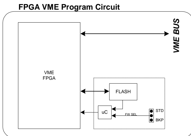
Fig. 3.4: FPGA VME diagram
