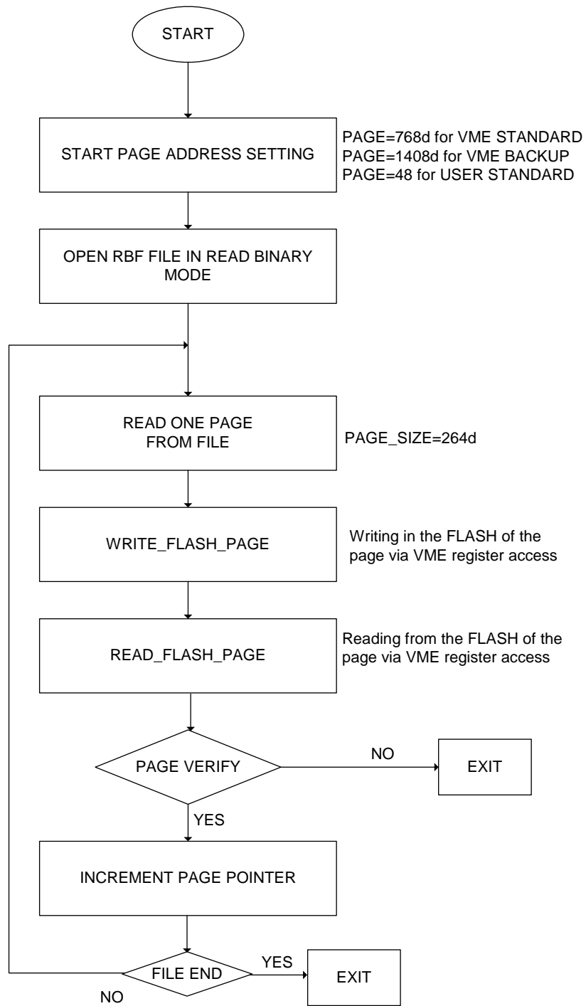
Fig. 5.16: Flash programming algorithm flow-chart
