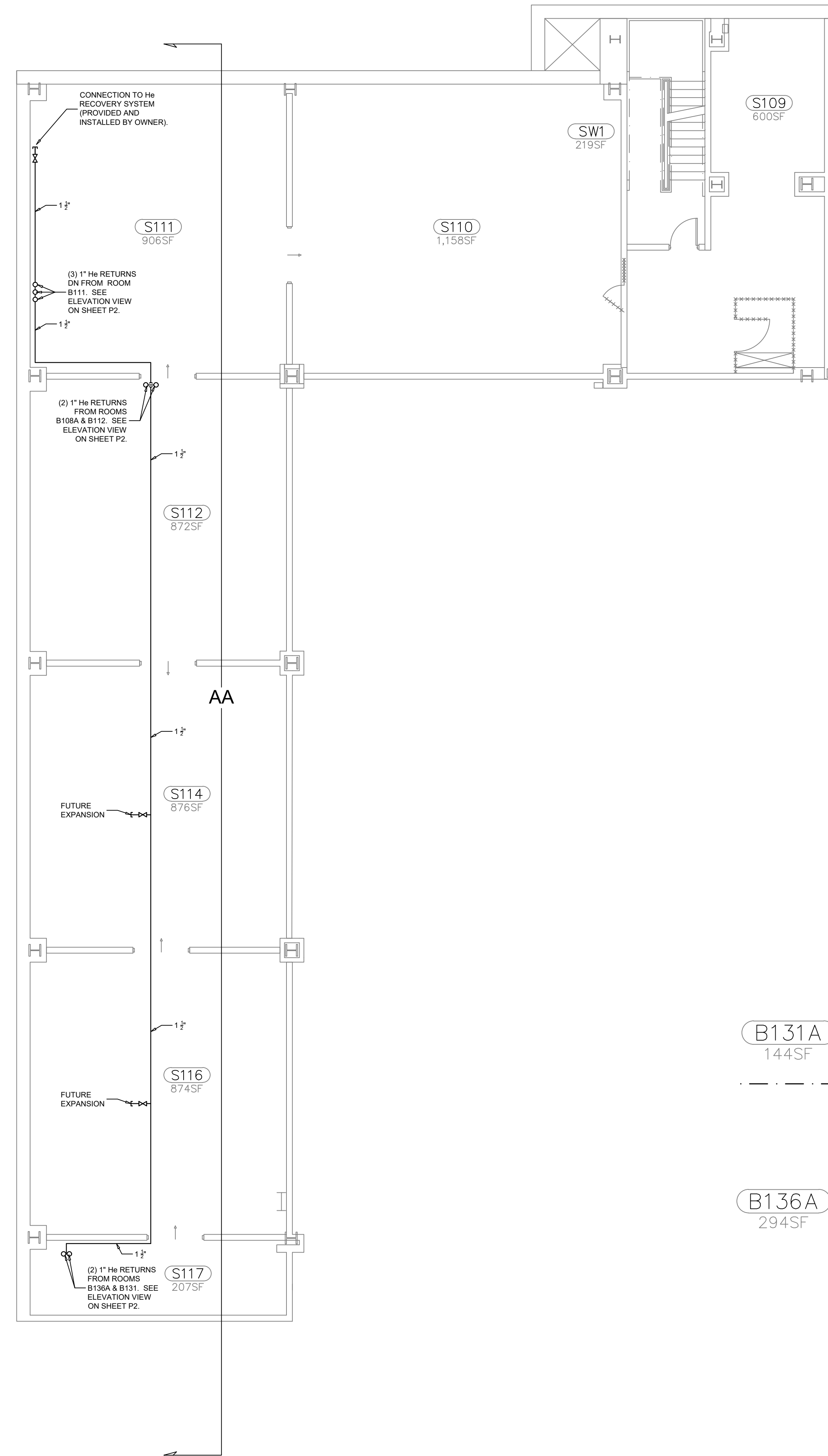
PLUMBING SUB BASEMENT FLOOR PLAN SCALE: 1/8" = 1'-0"
