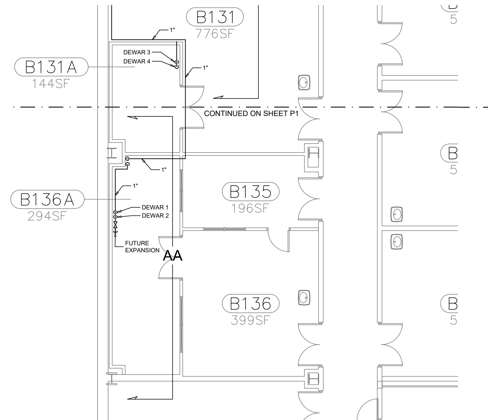
PLUMBING BASEMENT FLOOR PLAN SCALE: 1/8" = 1'-0"
