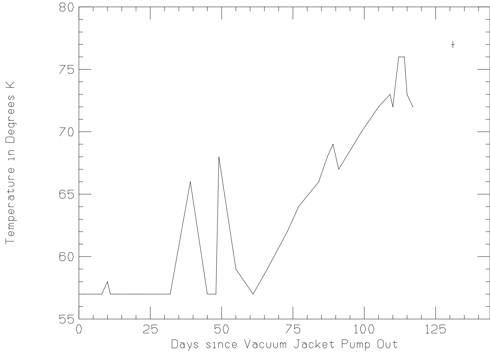
Purifier Cold Trap Temperature Since Vacuum Jacket Pump Out on 7-Apr-2023
