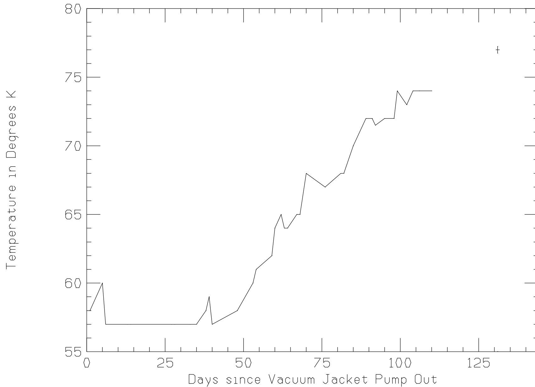
Purifier Cold Trap Temperature Since Vacuum Jacket Pump Out on 15-Dec-2022
