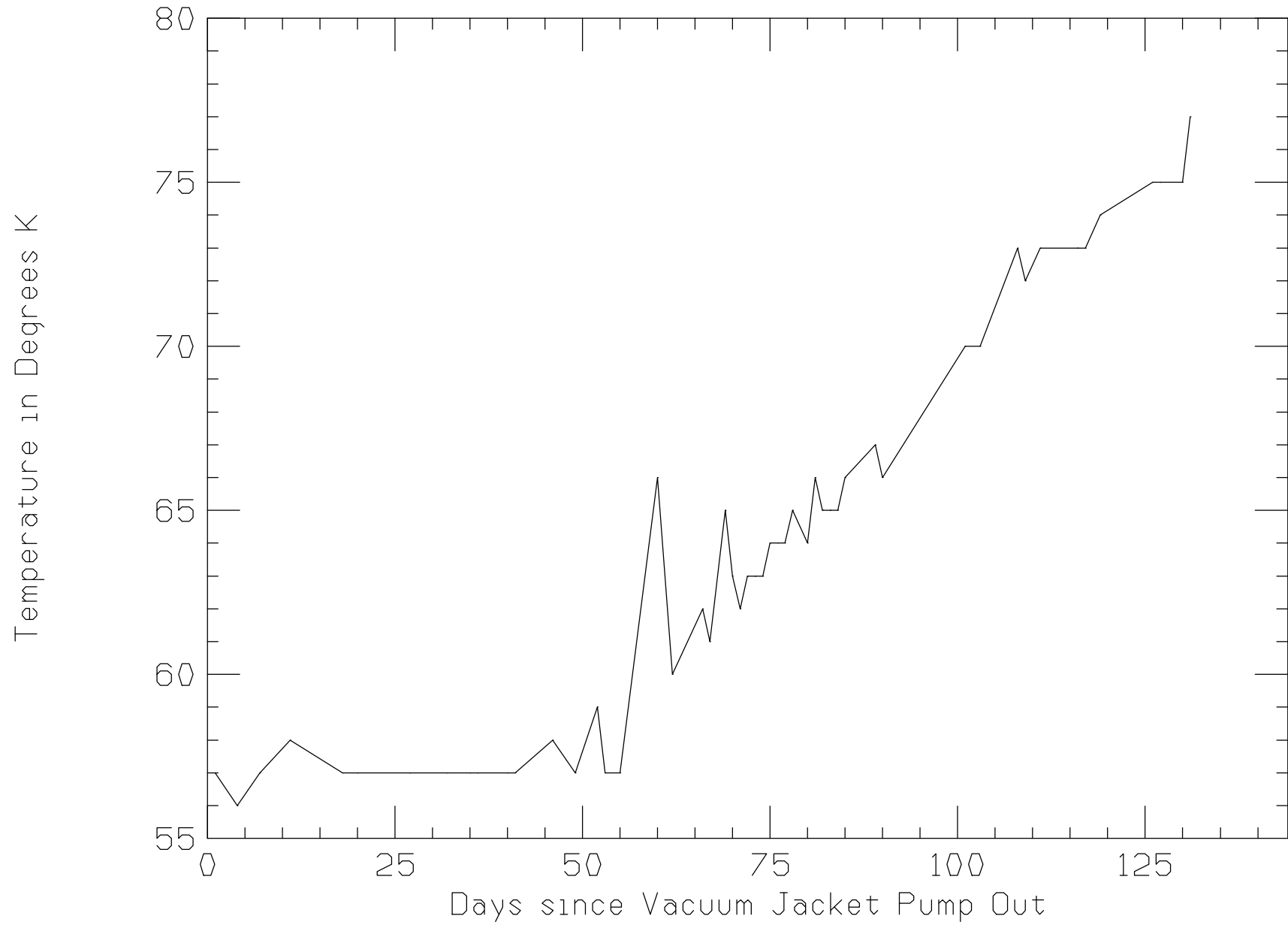
Purifier Cold Trap Temperature Since Vacuum Jacket Pump Out on 15-April-2022
